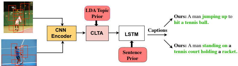
Fig. 1: Our Final Model with Conditional Latent Topic Attention (CLTA) and Sentence Prior (Sentence Auto-Encoder (SAE) regularizer) both rely on prior knowledge to find relevant words and generate non-template like and generalized captions compared to the same Baseline caption for both images - A man hitting a tennis ball with a racket.
