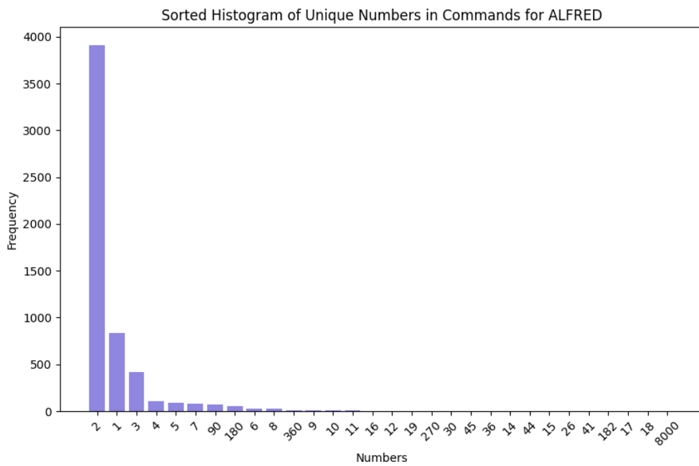
Figure 17: (A.2) ALFRED Numerics
