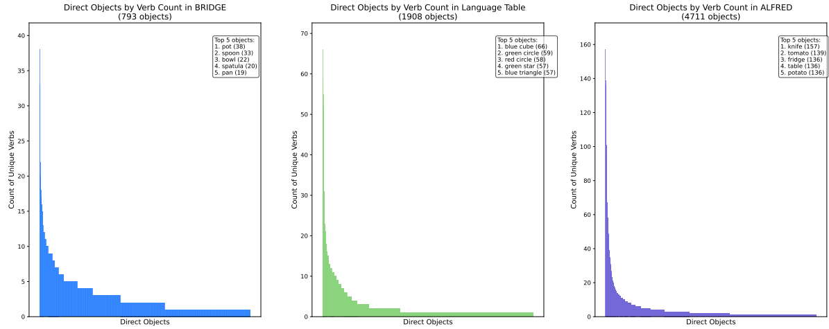
Figure 19: (A.2) Frequency Plot of Unique Verbs per Direct Object for Manipulation Datasets
