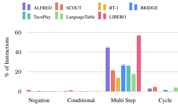
Figure 4: (A.3) Percentage of instructions exhibiting four structural phenomena: negation, conditionality, multi-step sequencing, and cyclic repetition. For datasets containing fewer than 600 unique sentences, annotations were performed manually. For those with more than 600 unique sentences, annotations were generated using an automated pipeline. Standard error bars reflect labeling uncertainty estimated from a manually reviewed subset of 500 randomly sampled commands per dataset.
