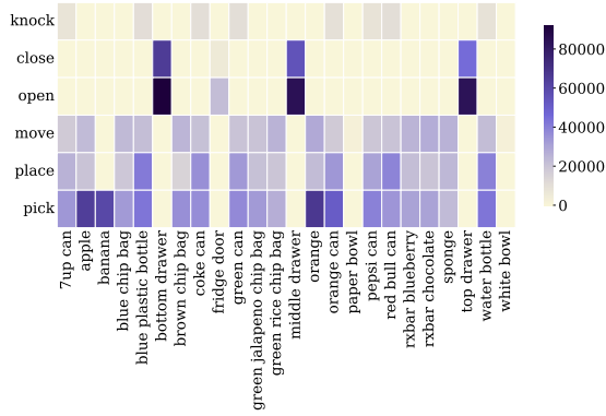
Figure 2: (A.2) Verb and direct object co-occurrence frequencies in the manually annotated RT-1 dataset. The heatmap highlights limited verb diversity across plausible actions; for instance, banana is frequently “picked” but never “moved.” The rare verb knock appears mostly with can-shaped objects, despite being equally applicable to others like an upright sponge.
