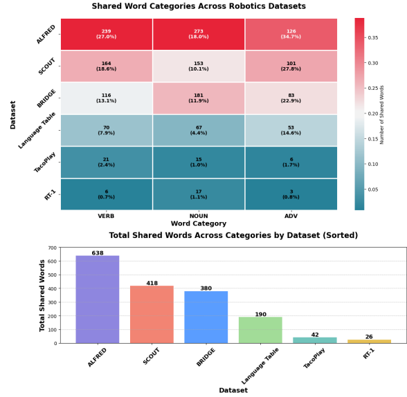
Figure 6: (A.1) Shared POS categories across datasets. Using ALFRED as a pretraining dataset is advantageous because it has the greatest amount of lexical coverage across the examined EAI datasets.
