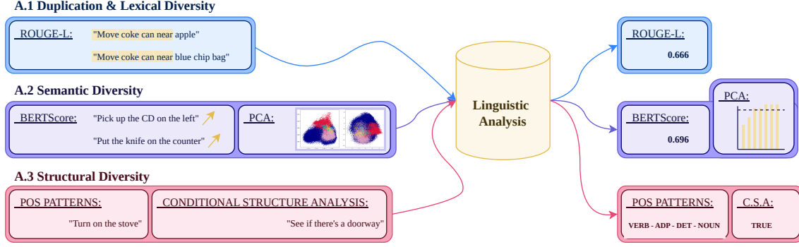
Figure 1: We analyze linguistic diversity in embodied AI datasets across three categories: A.1 Duplication & Lexical diversity, A.2 Semantic diversity, and A.3 Structural diversity.
