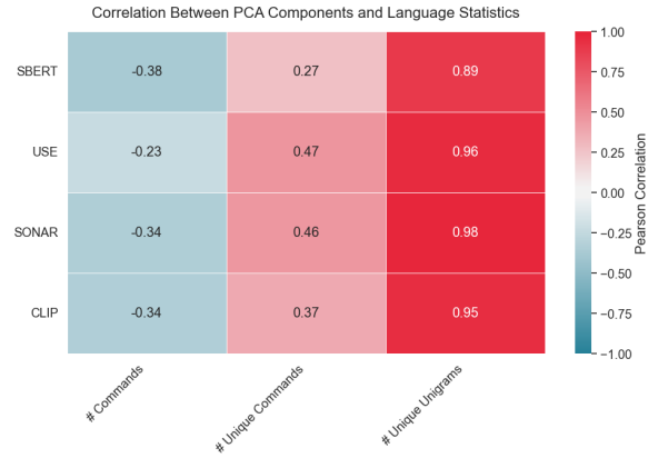
Figure 7: Correlation between the number of PCA components required to explain 95% variance and language statistics across EAI datasets. PCA components derived from SBERT, USE, SONAR, and CLIP embeddings are compared against the number of commands, unique commands, and unique unigrams in each dataset. Strong positive correlations are observed between unique unigrams and all embedding models, particularly SONAR and USE. In contrast, the total number of commands shows weak or negative correlation with embedding diversity.
