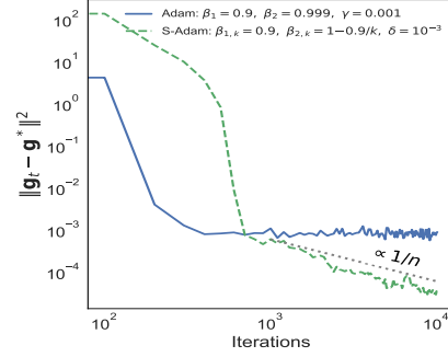
Figure 2: S-Adam outperforms Adam on Ex. 1, avoiding convergence plateau.
