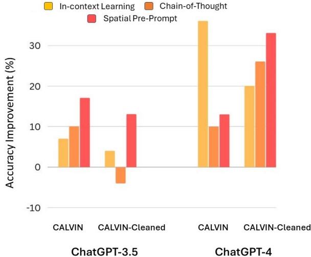
Figure 3: Accuracy Improvements (%) for In-context Learning, Chain-of-Thought and Spatial Prefix-Prompting on both the CALVIN and CALVIN-Cleaned datasets, for ChatGPT-3.5 and ChatGPT-4. As we can see, overall the accuracy gains for ChatGPT-4 are higher.
