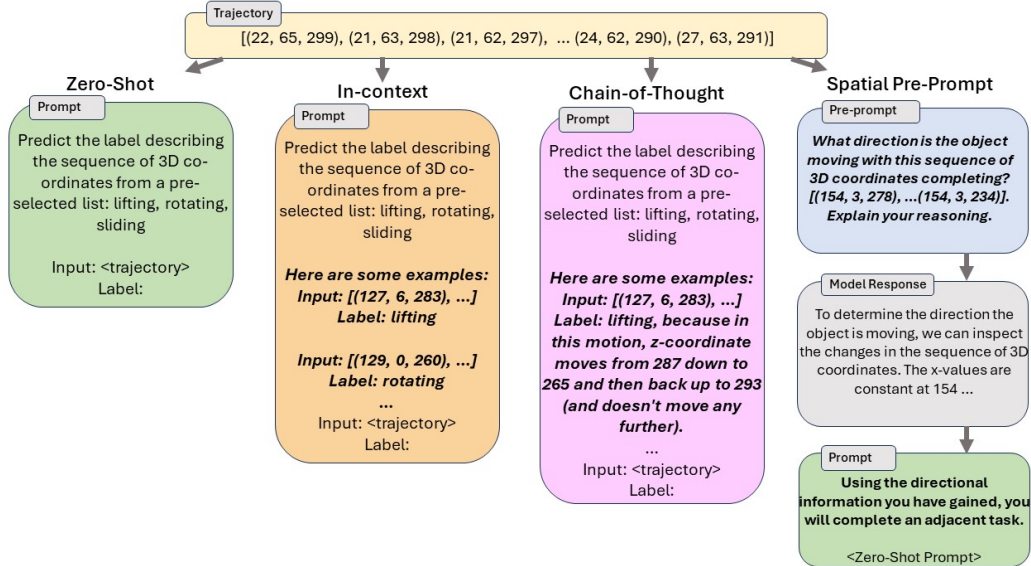
Figure 2: Different Types of Prompting Mechanisms - Zero-shot, In-context Learning, Chain-of-Thought and Spatial Prefix-Prompting. In Spatial Pre-Prompt, a tangential question is first asked, to which the model provides a response, following which the primary query is inquired.
