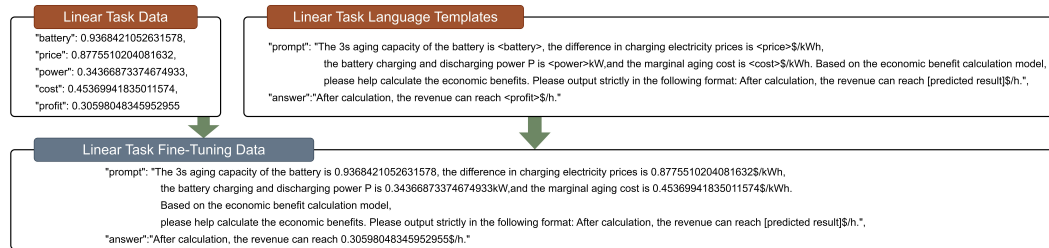
Figure 9: The combination of fine-tuning data for linear tasks, including calculation data related to profit and language templates.
