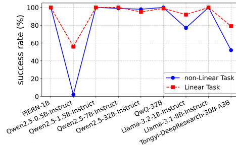
Figure 7: Success Rate between PiERN and multi-agent systems on inference tasks.
