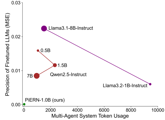
Figure 1: PiERN achieves high precision with low token usage. The horizontal axis represents the token usage of multi-agent systems with LLMs, and the vertical axis represents the precision of LLMs after finetuning.
