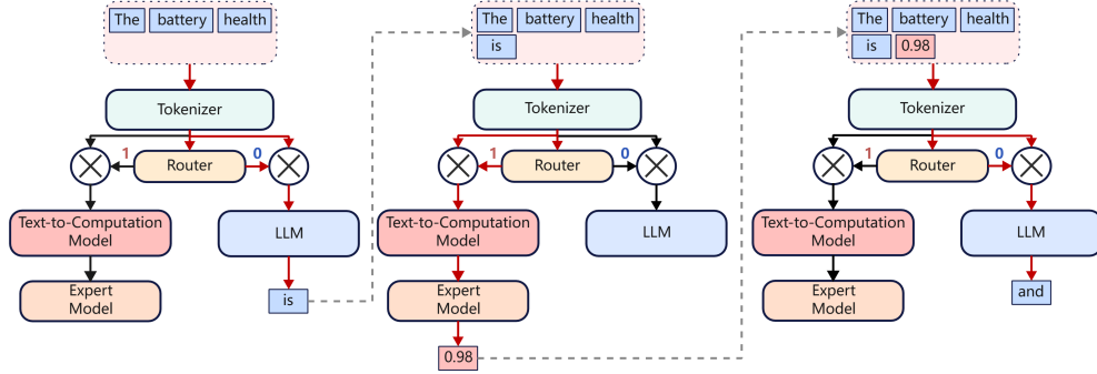
Figure 3: Token routing for reasoning-computation inference paradigm in PiERN. Left: Token Router decides to send tokenized inputs into LLM for generating the next token. Middle: Token Router decides to send tokenized inputs into the expert model for high-precision computation. Right: Token Router decides to send tokenized inputs with computation results to LLM for subsequent reasoning and planning.
