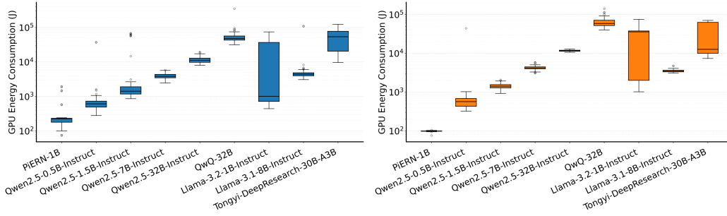
Figure 6: GPU energy consumption comparison between PiERN and multi-agent systems: (left) Non-linear battery capacity estimation task, (right) Linear battery profit calculation task.
