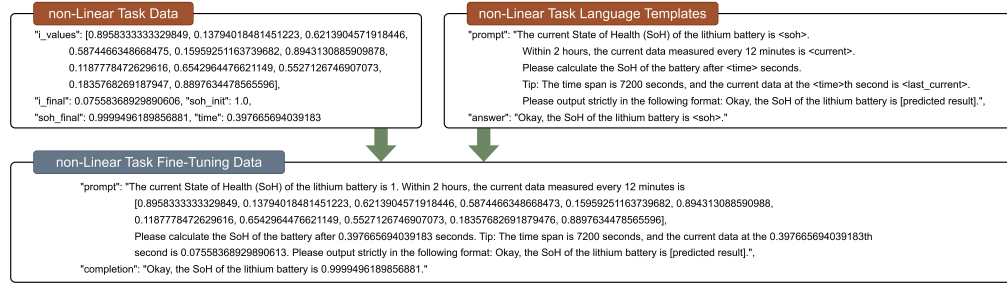
Figure 8: The combination of fine-tuning data for non-linear tasks, including time-series current data, time, battery health data, and language templates.
