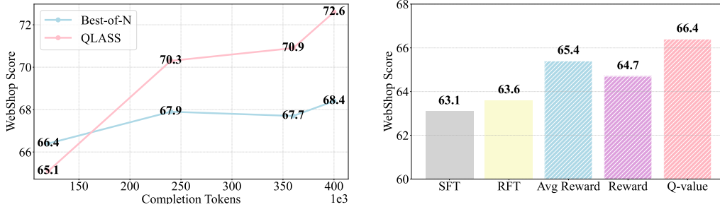
(a) QLASS and Best-of-N under different search budgets. The x-axis represents the number of tokens consumed by the trajectories generated during inference averaged on all the tasks in each test set. (b) Self-training baselines. The three methods marked with diagonal stripes leverage different process reward modeling based on the same exploration trees.
