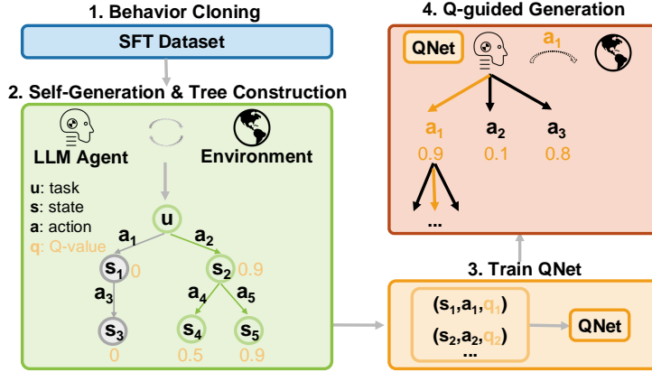
Figure 1: QLASS involves four stages: 1) Supervised fine-tuning (SFT) on expert data. 2) Leverage SFT agent to explore the environment and construct an exploration tree for each task. After construction, estimate the Q-value of each tree node based on Equation 7. 3) Train QNet on the estimated Q-values. 4) Use the trained QNet to provide inference guidance at each step.
