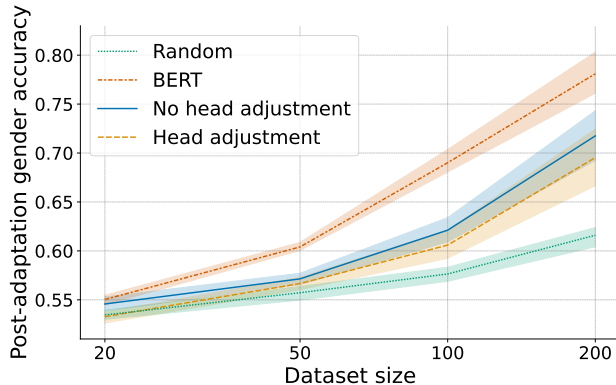
Figure 5: Ablating optimal adversary prediction calibration during MLAC training. Using optimally calibrated adversary predictions (modifying line 7 of Alg. 1) modestly improves blocking.
