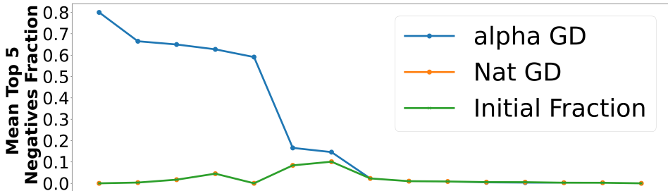
Figure 3: Fraction of negative values for natural versus \alpha gradient-based optimization across datasets. The X-axis represents datasets from ADbench (see Supplementary Material Section K for details).
