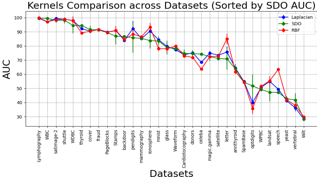
Figure 5: Comparing RSR results on ADBench for different kernel.
