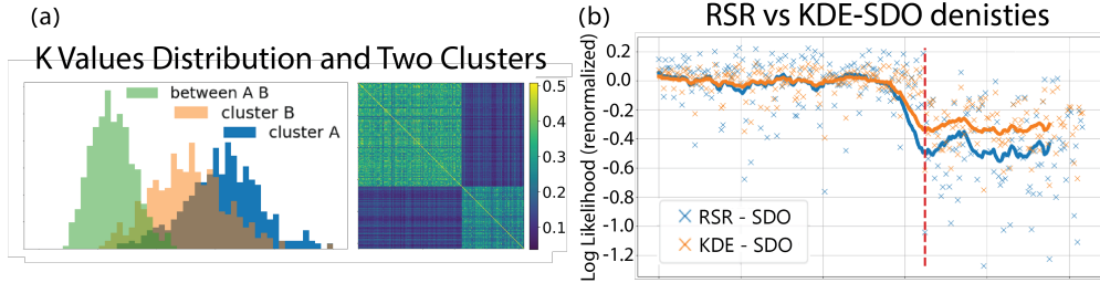
Figure 1: (a) Distribution of Kernel Values and SDO Kernel Values Inside and Between Clusters. (b) RSR and KDE Loglikelihoods. the x-axis represents points in the data, arranged by clusters, y-axis shows the log-likelihood.
