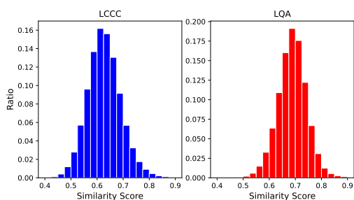
Figure 4: Similarity score distributions of LCCC (left) and LQA (right). The former is a chit-chat dataset and the latter is for QA scenario. The samples are generated by PanGu-Bot and the scores are calculated by BERTScore. Although overall scores of the chatting scene are lower, there are also some noise samples with much higher similarity scores for chit-chat and lower scores for QA.
