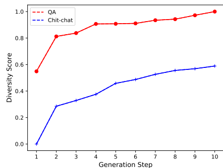
Figure 3: Token level diversity score (normalized) over generation steps.
