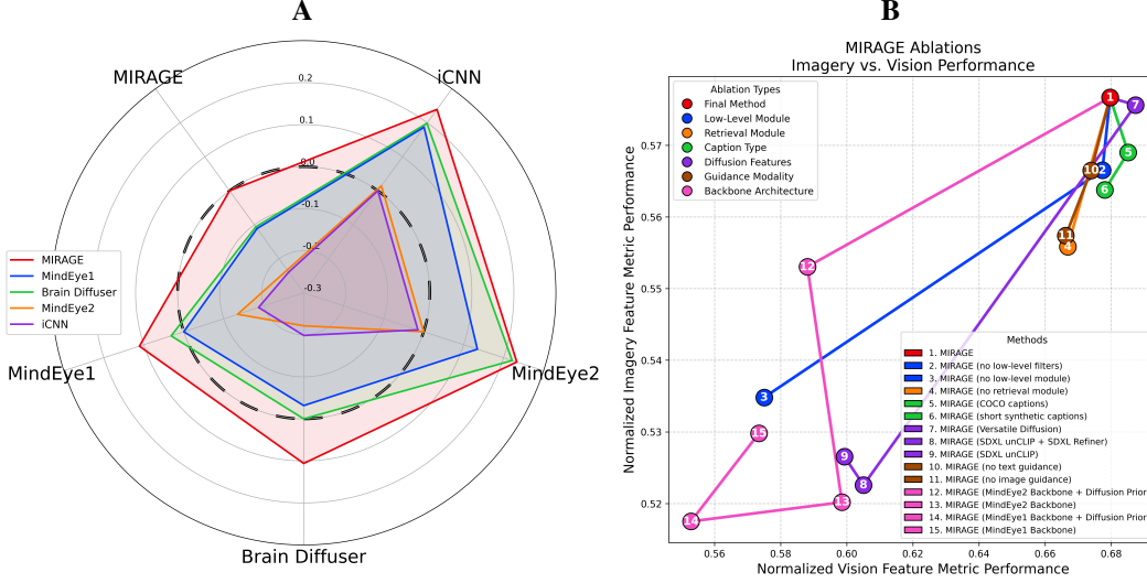
Figure 6: (A) Head-to-head human similarity score results for the conceptual stimuli. The Y-axis represents the similarity score advantage (difference between target method’s score and the alternative, on the radial X-axis); a larger colored polygon area indicates a stronger advantage, and the dashed circle at unity denotes equal performance. (B) Ablation analyses: model variants (numbered circles) under each ablation type (color) are assessed via the normalized average of all feature metrics (Table 1), with vision on the x-axis and imagery on the y-axis.
