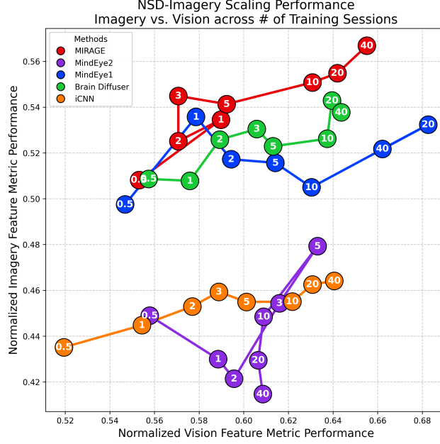
Figure 20: Performance of MIRAGE and other methods on NSD-Imagery for Subject 1 when trained on different numbers of fMRI sessions present in NSD. Each session includes approximately one hour of fMRI data. Metrics are the normalized average of all metrics in Table 1 of the manuscript, with imagery performance on the Y axis and vision on the X axis. Methods are indicated by color, with the number of training sessions indicated by the numbers in each dot.
