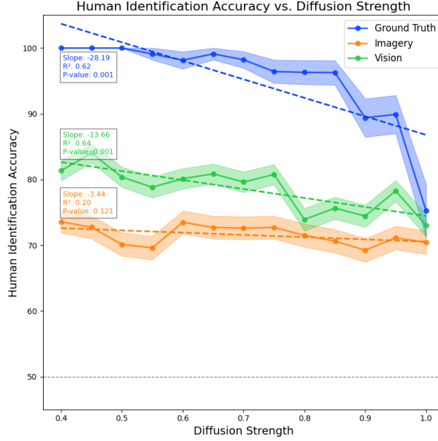
Figure 21: Human identification accuracy of MIRAGE (with no CLIP-Image guidance) as a function of diffusion model strength for imagery trials (orange line), vision trials (green line), and a control experiment that used the features directly from the ground truth image and caption (blue line). A dashed line is placed at the 50% chance threshold. Results are from a behavioral experiment that is identical to Experiment 1 (Table 5A), but varied across strength parameters.
