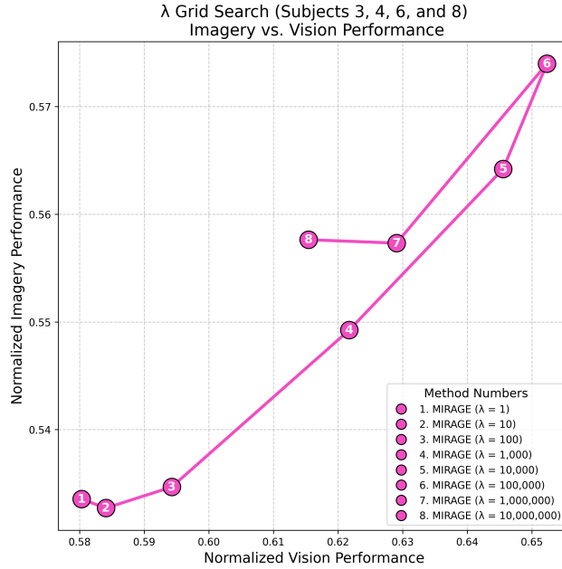
Figure 7: Hyperparameter logarithmic grid search over possible values of \lambda for use in Equation 1 (Section 3.3. Metrics are the normalized average of all metrics in Table 1 of the manuscript, with imagery performance on the Y axis and vision on the X axis.
