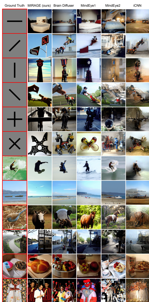
Figure 9: Median-case vision reconstructions from the vision trials of NSD-Imagery. Samples selected as median scoring based on metrics in Table 1 of the manuscript.
