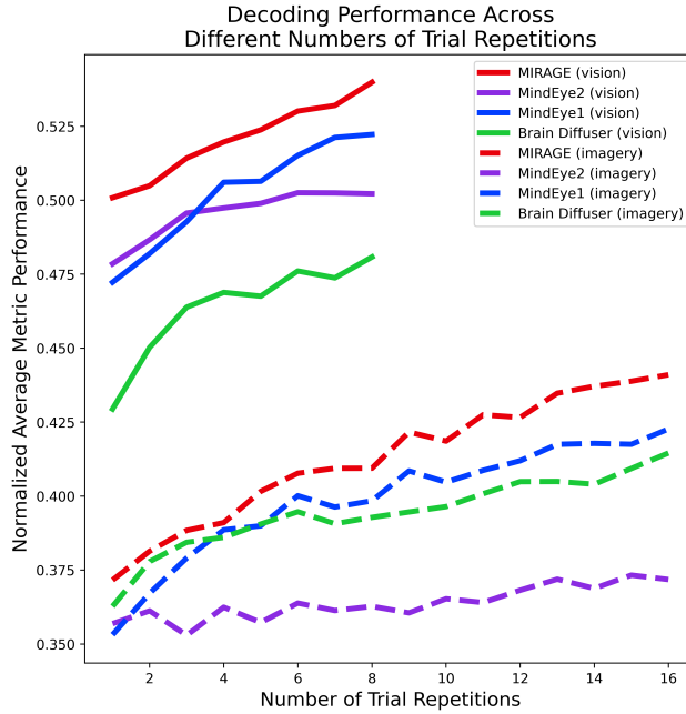
Figure 19: Performance of MIRAGE and other methods when averaging across brain activity responses to multiple trial repetitions of the same stimulus. Y-axis is the normalized average of all metrics in Table 1 of the manuscript, X-axis is the number of averaged trial repetitions.
