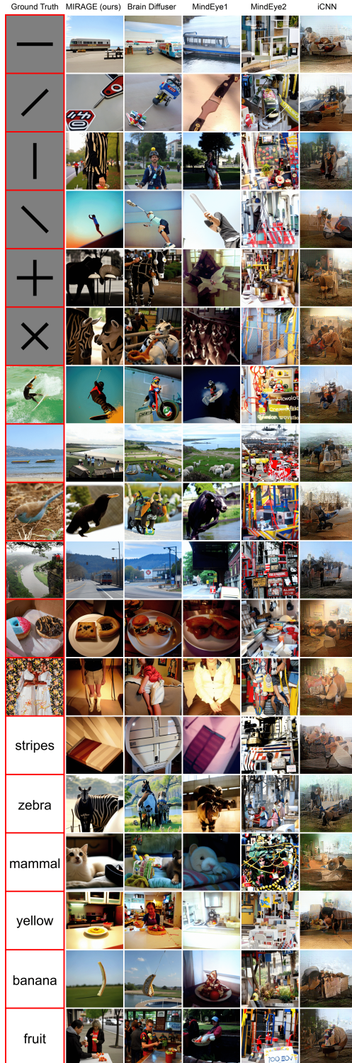
Figure 4: Qualitative comparison of reconstruction methods on imagined stimuli from NSD-Imagery. Reconstructions selected are the outputs sampled from each method and stimulus with the highest scores on all of the image feature metrics in Table 1. Examples from more methods can be seen in Appendix A.6.
