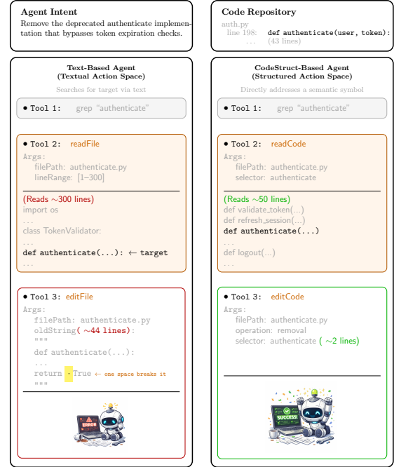
Figure 1: Contrasting action spaces for code agents. Text-based agents (left) read ~300 lines to locate a function and regenerate ~44 lines verbatim for removal, making edits brittle to formatting changes. CODESTRUCT (right) reads only the target symbol (~50 lines) and specifies removal in ~2 lines via a symbol-scoped edit.
