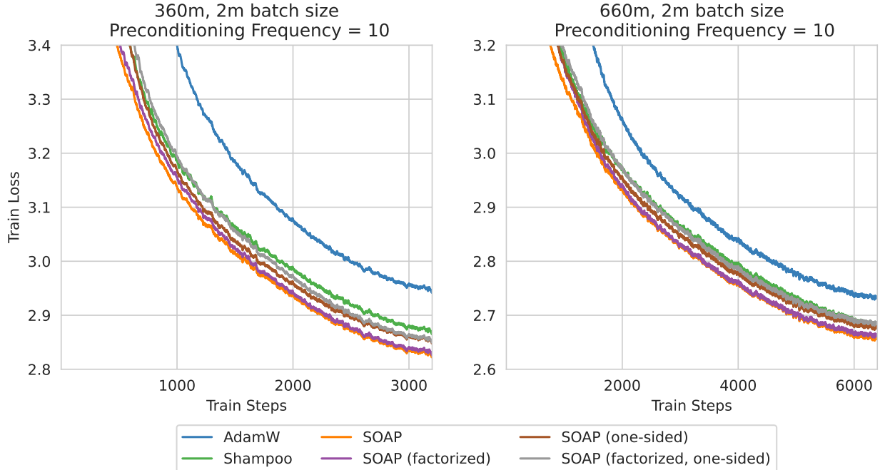
Figure 5: Performance of variants of SOAP which improve space usage or time overhead. 1. SOAP (factorized): Uses Adafactor instead of Adam in Shampoo’s eigenbasis and 2. SOAP (one-sided): Uses Q = I (i.e. no rotation) on the large side of weight matrix and 3. SOAP (factorized, one-sided): Combines both of these changes. We observe that while using Adafactor instead of Adam causes a negligible increase in loss, using the one-sided variant causes a larger increase. However, the one-sided variant also has much larger reduction in time and space overhead. For computational benefits of these variants see Appendices F.2 and F.3.
