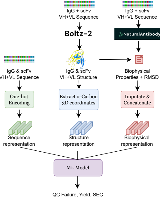
Figure 2: Multimodal ML pipeline.
