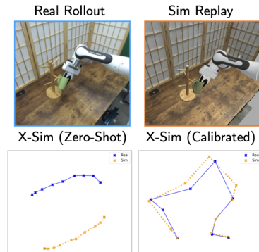
Figure 7: Sim-to-Real Calibration: We compare X-SIM image embeddings using t-SNE before and after calibration for one rollout.
