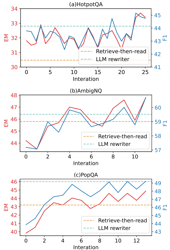
Figure 2: Reinforcement learning validation scores of (a)HotpotQA, (b)AmbigNQ, and (c)PopQA. The solid lines show EM (red) and F1 (blue) numbers through training iterations. The dashed lines are EM scores of the standard retrieve-then-read method (orange) and retrieval with an LLM as the rewriter (green).
