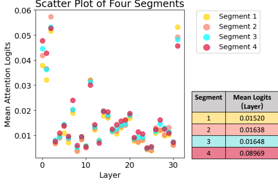
Figure 3: Scatter Plot of the average attention logits over 256 sentences at every layer. We divide the tokens into four segments based on token entropy, with segment 1 having the lowest entropy and segment 4 the highest. The figure indicates that as token entropy increases, so does the attention that the LLM allocates to that token.
