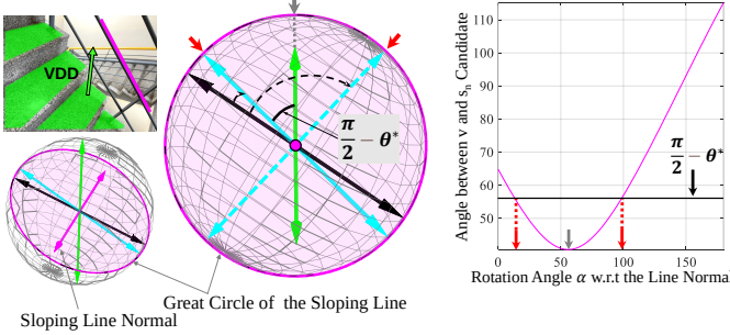
Fig. 10. Non-orthogonal method for SDD detection. The second column depicts the top view of the sloping line normal. Utilizing the property that a sloping line normal and the unknown-but-sought SDD are orthogonal, we parameterize SDD as s_n(\alpha) (cyan axis), which is the arbitrary vector u (black axis), lying on the great circle of the sloping line, rotated by an angle \alpha . We search for the \alpha where the rotated vector u makes an angle \frac{\pi}{2} - \theta^* with the VDD.
