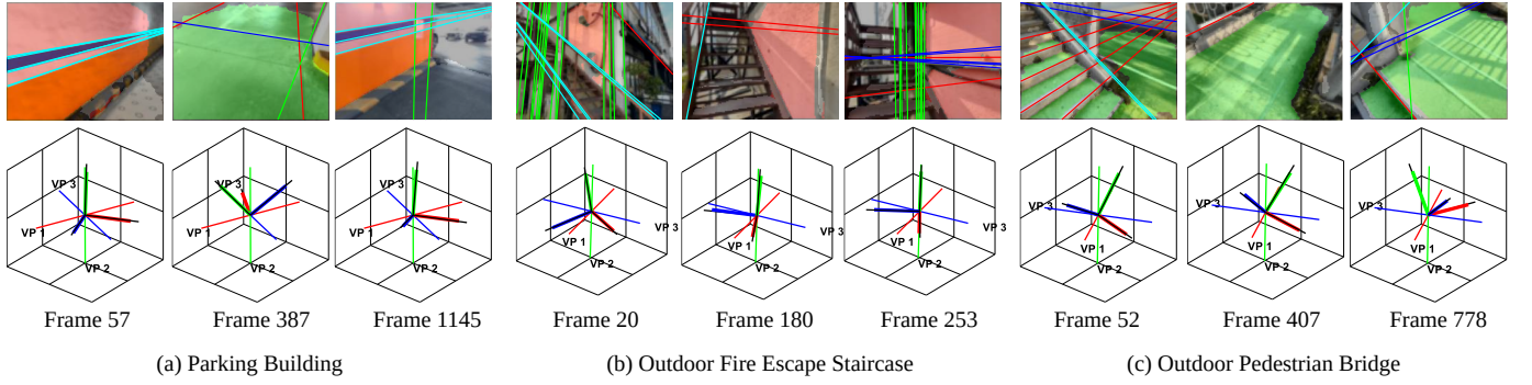
Fig. 14. Clustered lines and tracked dominant plane with inferred SFW frame are overlaid on the RGB images (top). Colored thick and thin lines denote the estimated 3-DoF camera orientation and the MW (VPs), and the black lines represent the true pose of the camera from Apple ARKit [23] (bottom).
