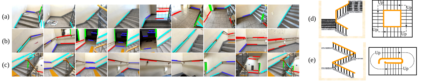
Fig. 11. Sample image sequences from our GIST-SFW dataset, the first indoor RGB-D dataset in SFW, with line clustering results from the proposed method. We capture sequence (a) on a quarter-turn staircase illustrated in (d). We capture sequences (b) and (c) on a half-turn staircase illustrated in (e). We establish and release the GIST-SFW dataset for the evaluation of the proposed SLOPe and other methods in SFW.
