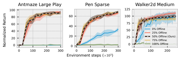
Figure 12. RLPD is not sensitive to replay proportion; 50% offers the best compromise between variance, speed of convergence, and asymptotic performance.
