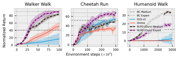
Figure 5. Our approach generalizes to vision-based domains, providing consistent improvements over existing approaches.
