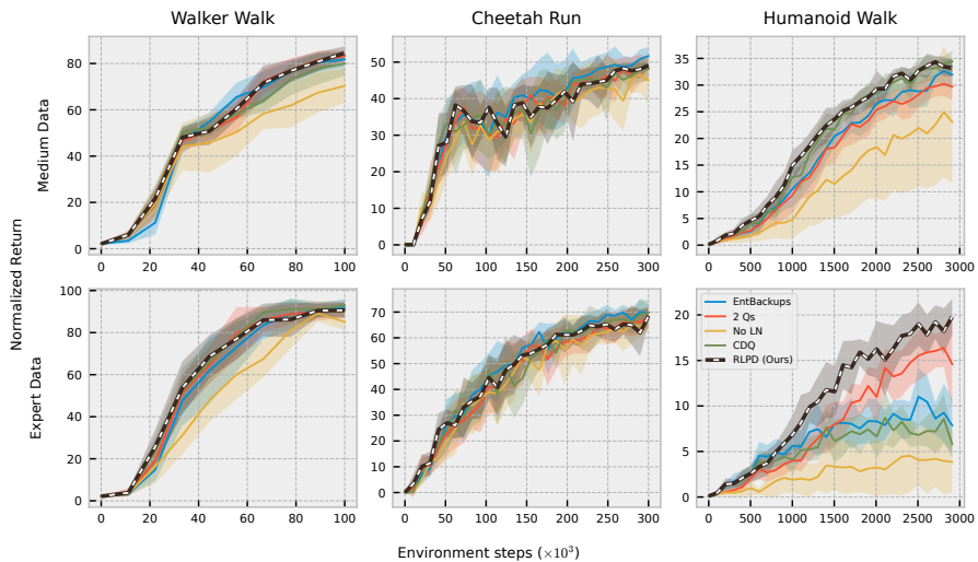
Figure 20. VD4RL Ablations.
