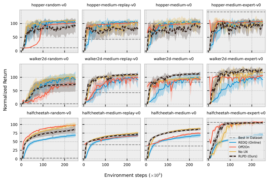
Figure 18. D4RL Ablations.
