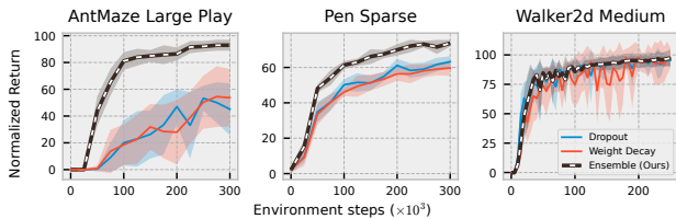
Figure 9. In general, critic ensembling provides the best performance. Dropout performs worse in sparse reward tasks.
