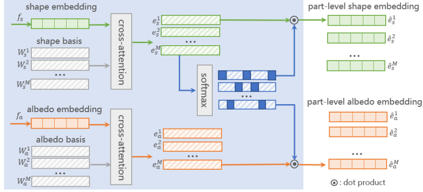
Figure 2: Illustration of the Graphics Decomposition Module (GDM). GDM is proposed to ensure that each part capsule presents a semantic consistent part of objects.
