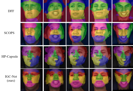
Figure 8: The qualitative comparison of unsupervised face segmentation on BP4D.
