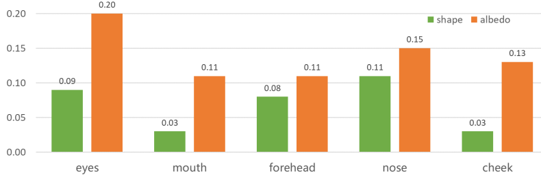
Figure 4: The importance of part-level graphics capsules for face recognition. On average, the albedo is more crucial than the shape when recognizing faces. The albedo of the eyes is the most important component and the shape of the nose is more important than the shape of other parts.
