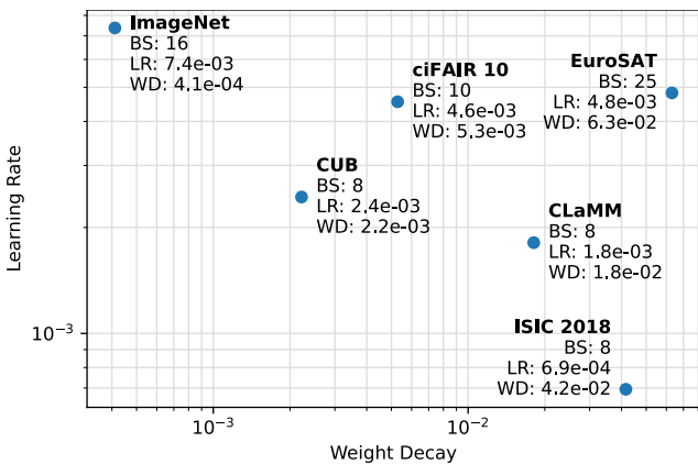
Figure 3: Hyper-parameters found with ASHA [16] for the cross-entropy baseline. BS = batch size, LR = learning rate, WD = weight decay.
