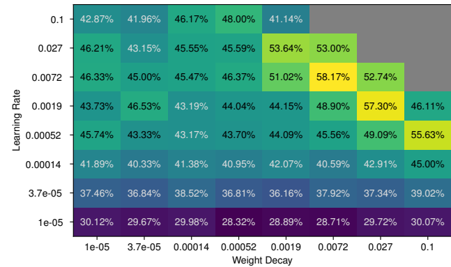
Figure 1: Classification accuracy obtained with standard cross-entropy on ciFAIR-10 with 1% of the training data for different combinations of learning rate and weight decay. Gray configurations led to divergence.
