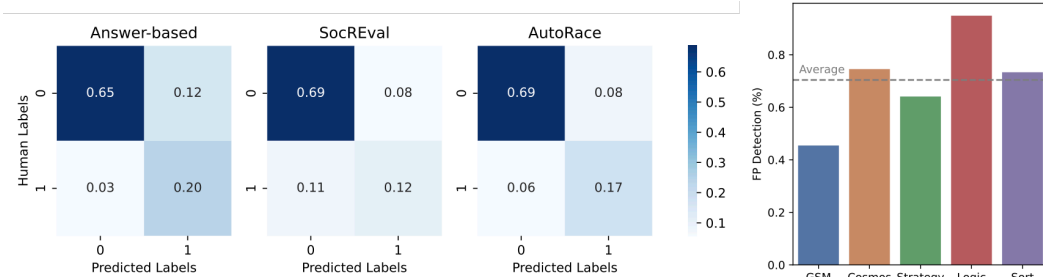
Figure 3: Analysis on different reasoning chain evaluation methods: (Left) The macro-averaged confusion matrix of these methods. SocREval and AutoRace are both good at detecting incorrect reasoning chains, while SocREval mistakenly classifies correct reasoning chains as wrong more frequently. (Right) AutoRace can recognize 70.4% of the false positive reasoning chains, showing the promise to be a great complement to answer accuracy.
