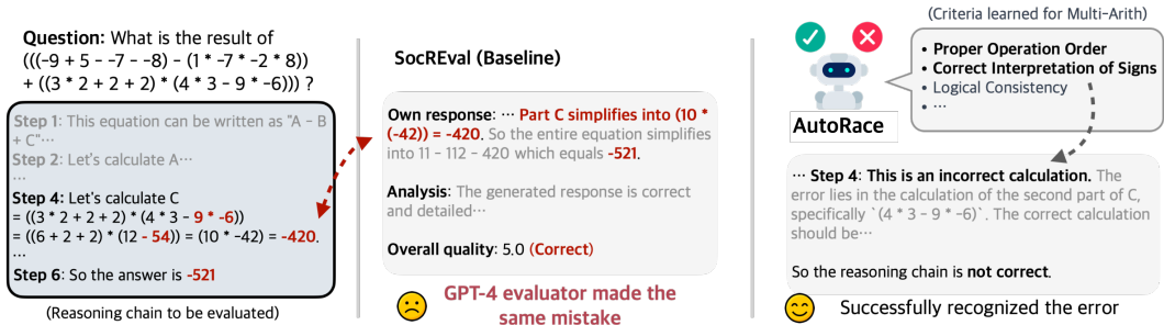
Figure 6: A case study on MultiArith (Srivastava et al., 2023). SocREval (He et al., 2023) requires GPT-4 to generate its own response to the problem, and then use it as the reference to evaluate the reasoning chain. In this case, it makes the same mistake as the reasoning chain. AutoRace successfully recognized the calculation error, guided by the criterion list learned for this task.
