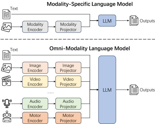
Figure 1: Overview of modality-specific language models and Omni-modal language models.
