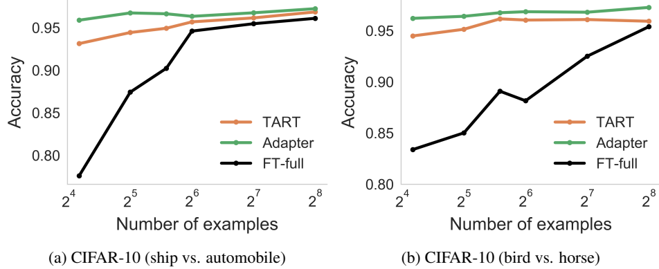
Figure 28: Additional CIFAR-10 binary classification tasks. TART is competitive with task-specific full fine-tuning and adapters.
