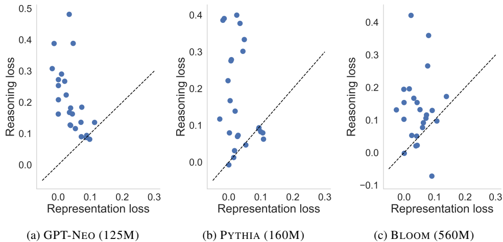
Figure 12: Effects of fine-tuning on task-agnosticity . Scatter plot of reasoning loss against representation loss when the base model is trained on AG-News-0 and evaluated on other tasks. Across datasets (each point in plot represents a dataset), fine-tuning majorly impairs reasoning when transferring to tasks outside the specific fine-tuned task.
