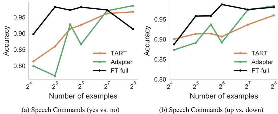
Figure 29: Additional Speech Commands binary classification tasks. TART is competitive with task-specific full fine-tuning and adapters.
