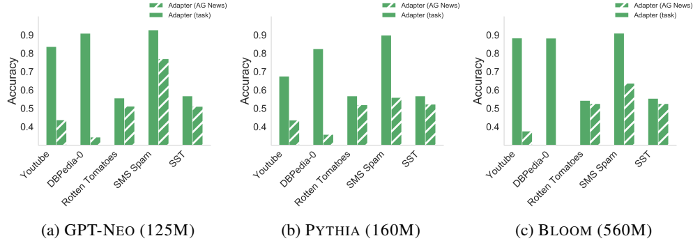
Figure 13: Effects of fine-tuning on task-agnosticity of adapters. Accuracy of task-specific fine-tuned adapter vs. accuracy of adapter fine-tuned on AG-News-0 and evaluated on task. Fine-tuning consistently hurts the generalization ability of adapters across datasets.
