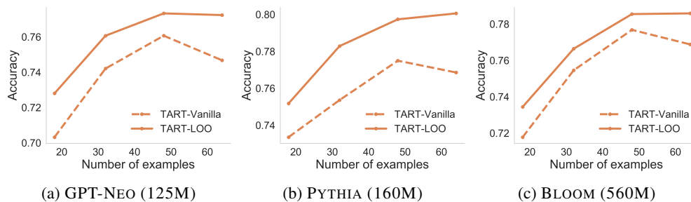
Figure 16: LOO embeddings vs. Vanilla Embeddings. Comparison of TART performance when using LOO embeddings and vanilla embeddings. Vanilla embeddings see a performance collapse, but LOO embeddings do not.
