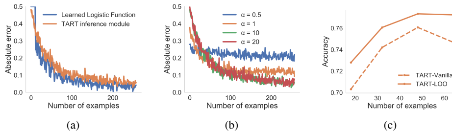
Figure 18: Properties of TART’s inference module. (a) Comparison with learned logistic function: inference module recovers underlying probabilities. (b) Variation in error with different noise levels for model trained on \alpha = 10 . (c) Comparison of TART performance when using LOO embeddings and vanilla embeddings.
