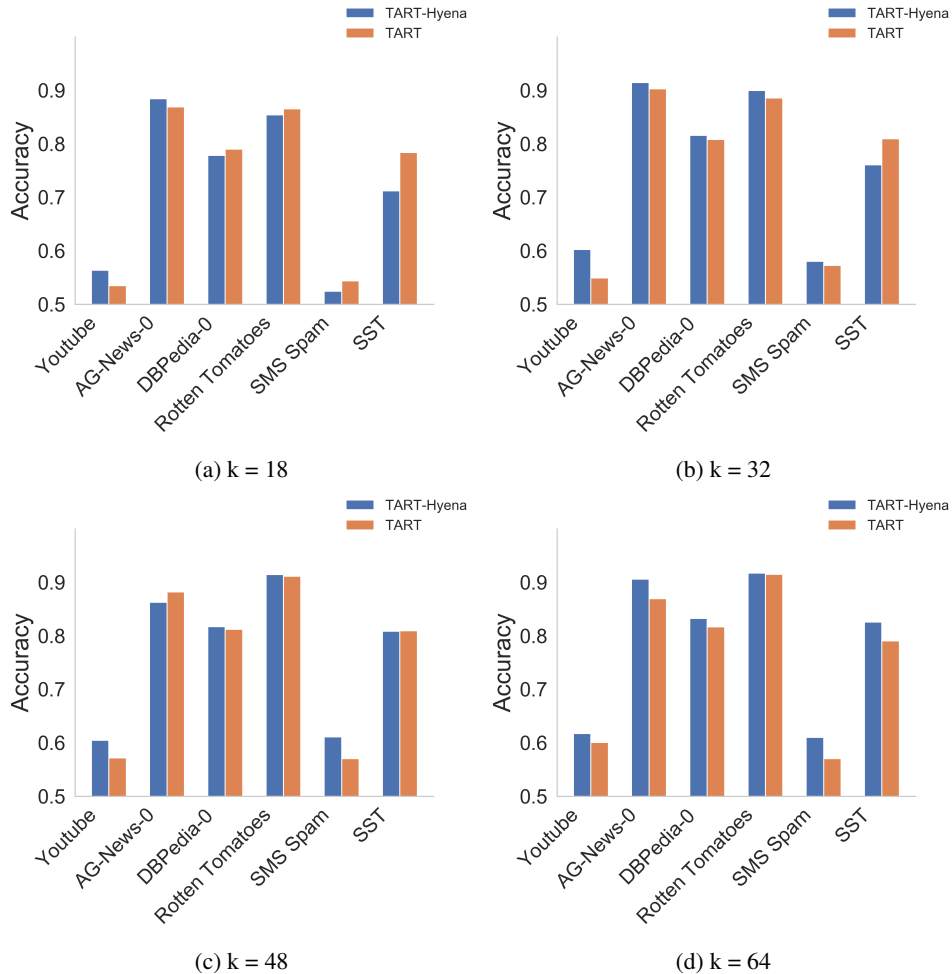
Figure 25: Comparing TART with a Hyena version of TART. Instead of using a Transformer module, we use a Hyena model to learn the probabilistic reasoning task. Hyena-TART is comparable to TART across datasets and achieves better performance for larger value of k ( = 64 ).
