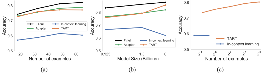
Figure 4: Effects of scale. (a) Effect of number of in-context examples on performance for different task adaptation strategies. (b) Effect of model size on the performance of different task adaptation strategies. (c) Beyond context length limitations, performance comparison with respect to number of in-context examples.
