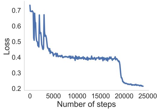
Figure 15: Training loss vs. number of steps. The plot shows the variation in training loss as a function of the number of steps of gradient descent for TART’s reasoning module.
