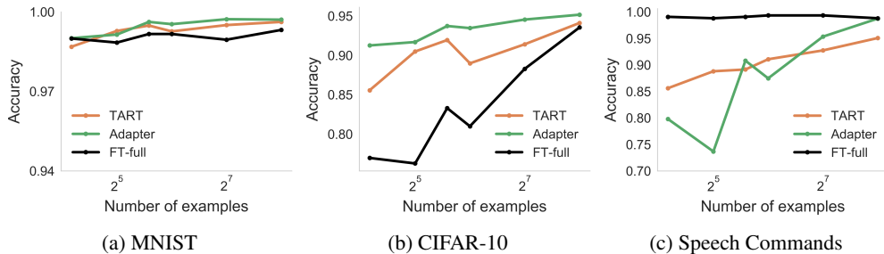
Figure 5: TART can generalize across domains using the same inference module that was used for language benchmarks: Performance across vision tasks (MNIST, CIFAR-10) and an audio task (Speech Commands).
