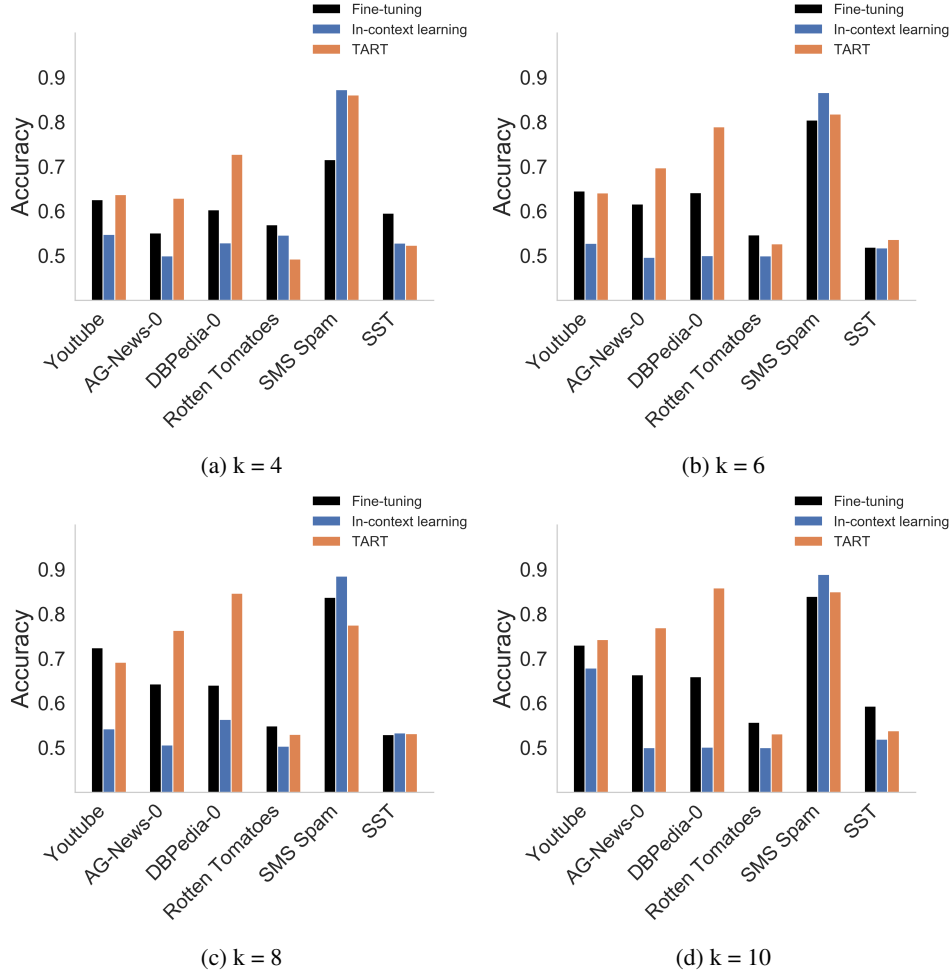
Figure 26: TART in low sample regime
