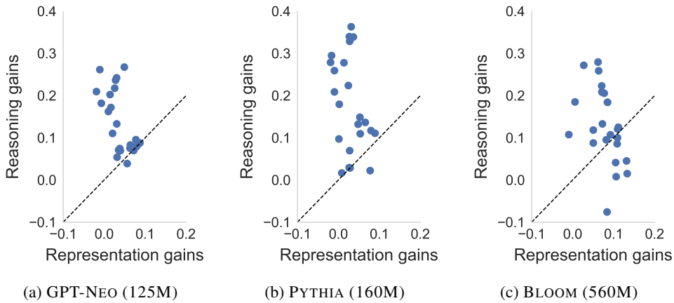
Figure 9: Effects of fine-tuning on reasoning. Across datasets (each point in plot represents a dataset) and model families, fine-tuning improves task-specific reasoning which improves its performance over base in-context learning.
