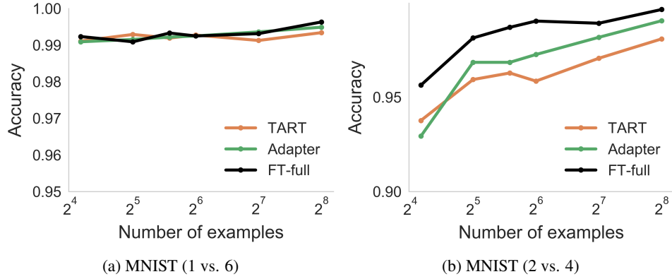
Figure 27: Additional MNIST binary classification tasks. TART is competitive with task-specific full fine-tuning and adapters.
