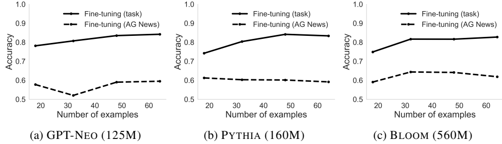
Figure 10: Effects of fine-tuning on task-agnosticity Accuracy of task-specific fine-tuned model vs. accuracy of model fine-tuned on AG-News-0 and evaluated on task. Fine-tuning hurts task-agnosticity across all three model families.
