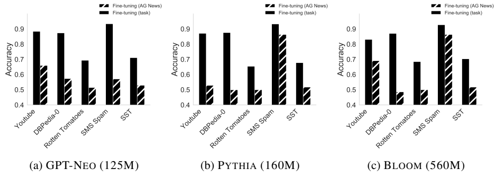
Figure 11: Effects of fine-tuning on task-agnosticity (dataset level) Accuracy of task-specific fine-tuned model vs. accuracy of model fine-tuned on AG-News-0 and evaluated on task. Fine-tuning consistently hurts task-agnosticity across all three model families and datasets.
