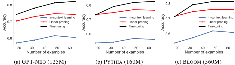
Figure 7: Comparison of linear probing, in-context learning, and fine-tuning. Accuracy of in-context learning vs. linear probing on model embeddings across three model families: representations have sufficient information.
