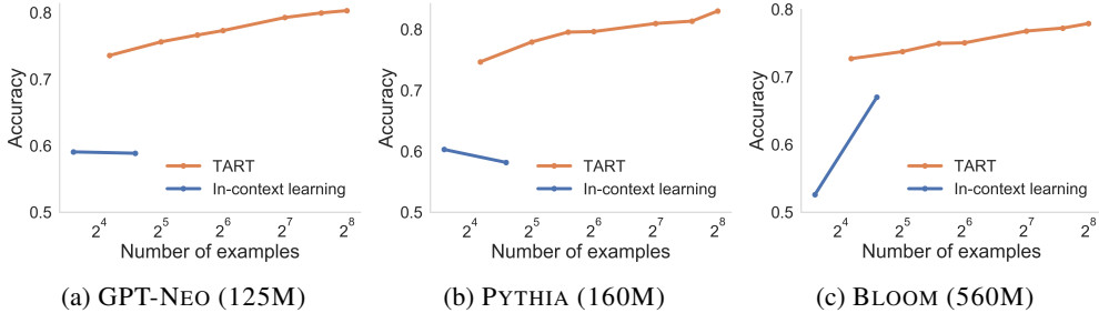
Figure 23: Beyond context window constraints . Performance comparison with respect to number of in-context examples. Base in-context learning is bound with respect to total numbers of examples and performance saturates. TART is not bound by context length, and performance continues to scale as number of examples increases.
