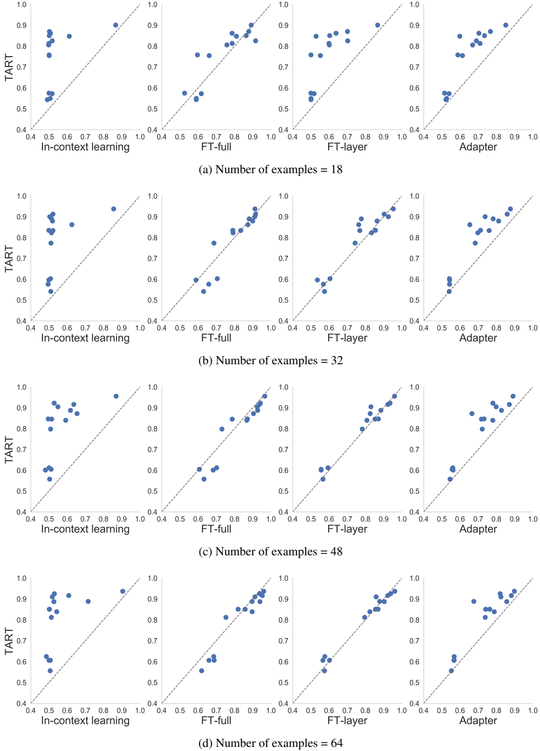
Figure 21: Comparison of TART and task-adaptation approaches (PYTHIA (160M)). We see that for PYTHIA (160M), TART outperforms in-context learning and adapters and is competitive with full fine-tuning across all k .
