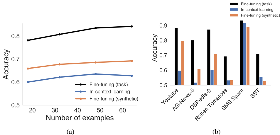
Figure 6: Fine-tuning with NL synthetic task. (Left) Averaged over 6 different tasks, fine-tuning with the NL synthetic task provides a lift over base in-context learning, and scales with number of examples. (Right) Dataset level comparisons between task-specific fine-tuning, in-context learning and synthetic fine-tuning: synthetic fine-tuning outperforms base in-context learning on 4 out of 6 datasets, but lags task-specific tuning.
