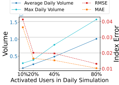
Figure 15: Scaling law: Performance \propto Volume.
