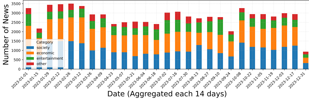
Figure 26: The x-axis indicates the date, and each bar represents the distribution of the average number of news for each topic over a 14-day period beginning with that data.
