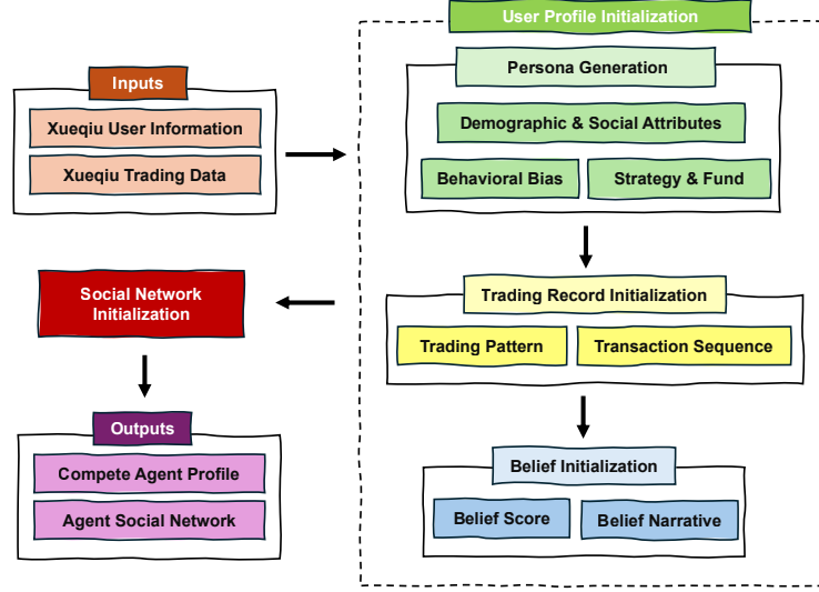
Figure 28: Pipeline of User Profile Initialization.
