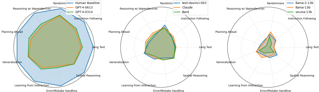
Figure 3: Left: comparing the two GPT-4 variants with Human Baseline performance as reference. Middle: comparing text-davinci-003, Claude, and Bard. Right: comparing open-source llama-2-13b, llama-13b, vicuna-13b models.
