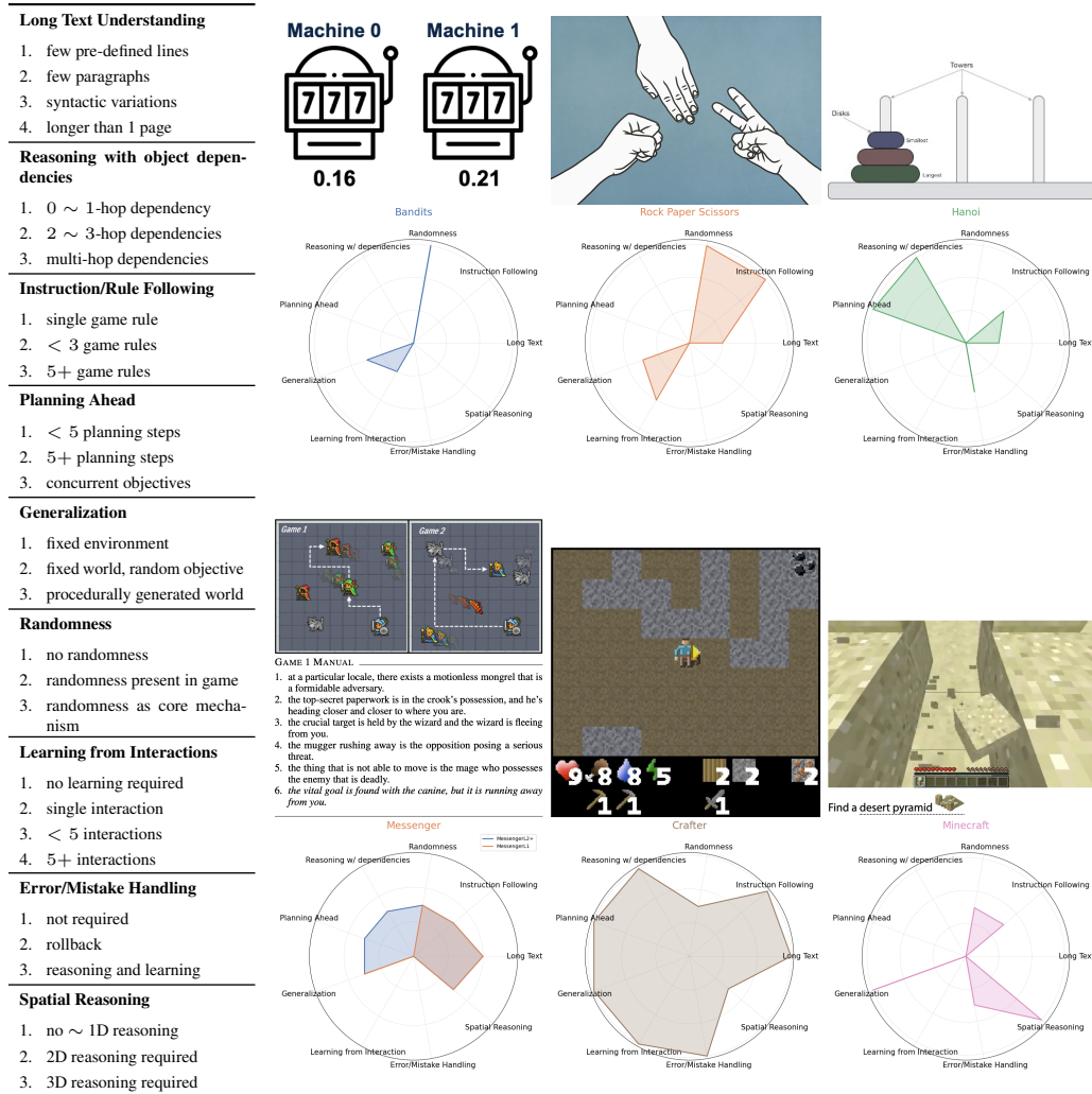
Figure 2: We identify a set of 9 important capabilities for an intelligent agent. We identify different degrees of challenge for each capability as shown on the left. Each game in SmartPlay challenges unique set of capabilities at different degrees, as shown in the spider charts. We numerical values for the spider plots in Table 3.
