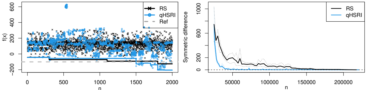
Figure 5: Left: optimality gap for the Lunar lander problem (one single run) with the evaluated values and estimated minimum found. Right: results on CityCOVID data set over 5 macro-runs, thin dashed lines are 5% and 95% quantiles.
