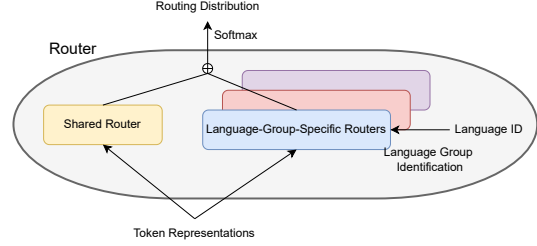
Figure 2: Diagram of the proposed language group router.
