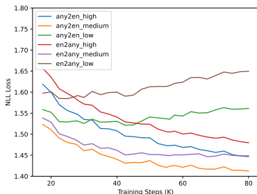
Figure 5: The validation loss of the MMNMT model during training.
