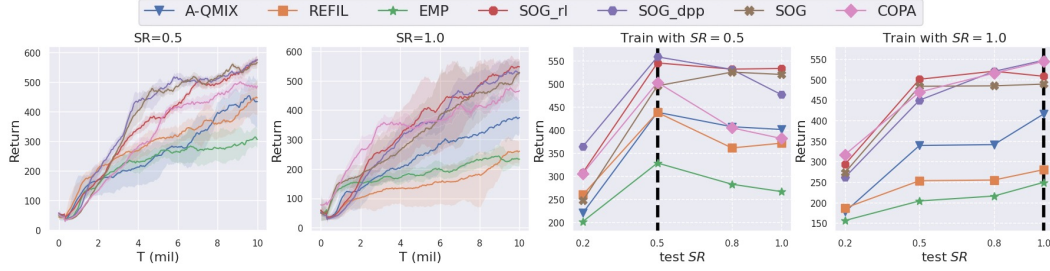
Figure 4: (a-b) The average episode returns in the scenario Resource Collection with 2 kinds of sight ranges (SR). (c-d) Their performance on different test sight ranges from SR = 0.2 to SR = 1.0 .
