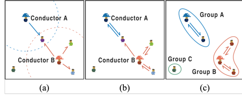
Figure 2: The process of group organization. (a) Conductors are elected, and send group invitations to the neighbors. (b) Followers choose the conductor and send the summarized messages. (c) Groups are formed and conductors send unified targets to the group members.
