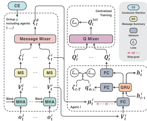
Figure 3: A diagram of the model structure. “MHA” means multi-head attention. We use this module to deal with the entity-wise input for dynamic team composition, detailed in Appendix A. h_t^i is the hidden state for GRU cell.
