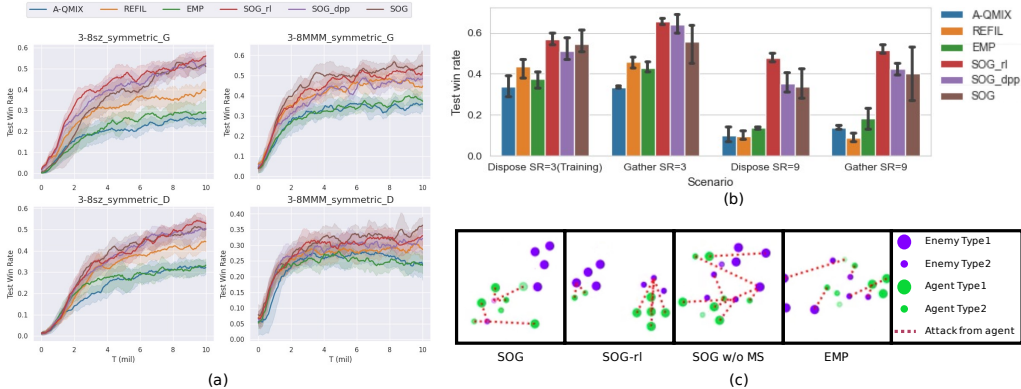
Figure 5: (a) Results of the test winning rates on StarCraft2. (b) Models’ performance when transferred to unseen scenarios. (c) Visualization of agents’ behaviour at time step 20.
