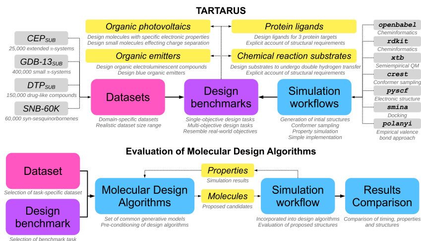
Figure 1: TARTARUS framework, highlighting its two core elements. Top: Real-world design tasks are defined and paired with simulation workflows and datasets. Bottom: The Evaluation Pipeline: Generative models are conditioned using reference datasets, sampled for structures, and evaluated based on their properties through custom simulation workflows. Model performance is assessed based on the alignment of the acquired properties with predefined objectives.
