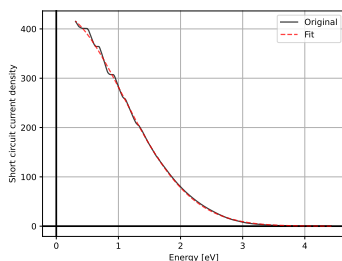
Figure S6: Short circuit current density as a function of the band gap energy of the light-absorbing material in an organic solar cell. The original dependency results from the integration of the Reference Air Mass 1.5 Spectra (AM1.5G). The fit depicts the result of regression with a Gaussian function with two fitting parameters.
