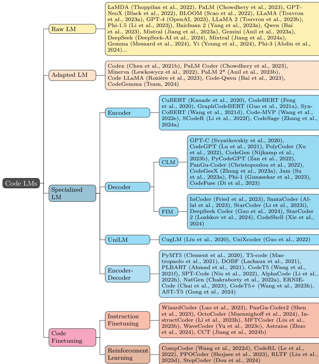
Figure 1: Our taxonomy of pretrained language models for code.
