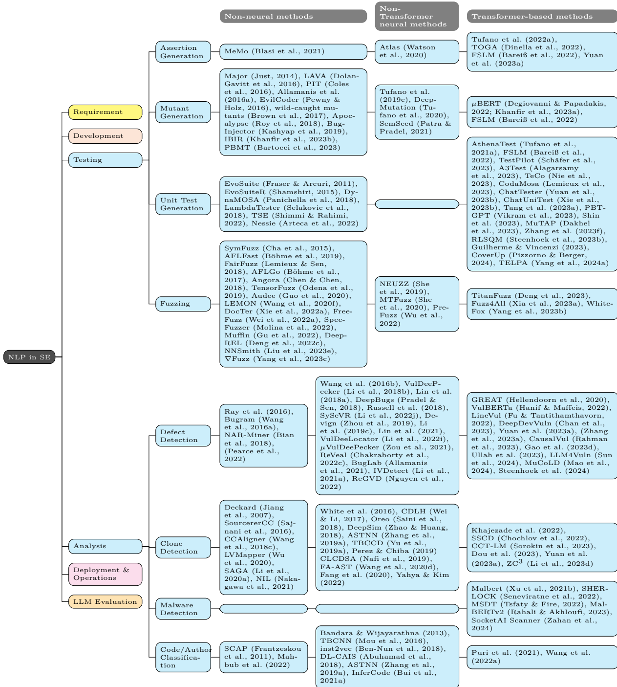
Figure 6: NLP applications in the testing &amp; analysis stage of SE.
