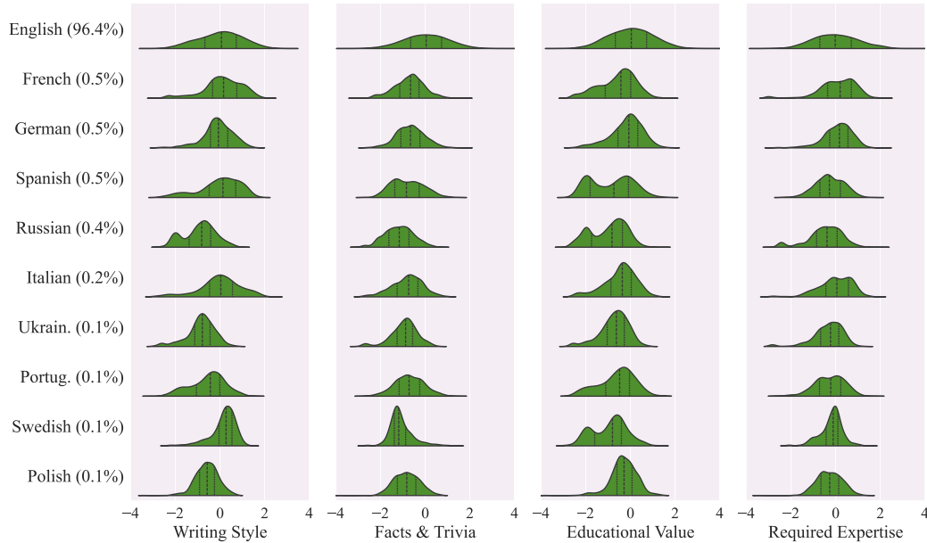
Figure 4: Distribution of quality ratings for the 10 most common languages in 1M documents randomly sampled from SlimPajama, normalized for each criterion to have zero mean and standard deviation.
