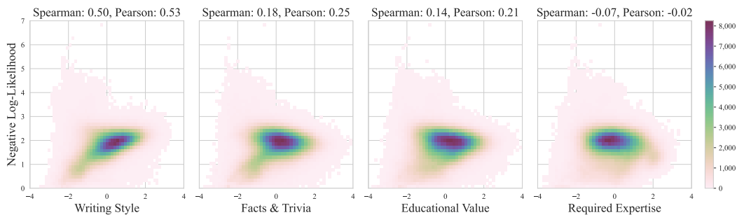
Figure 5: Correlations of quality ratings and negative log-likelihood scores by Llama-2-7B(Touvron et al., 2023b) over 1M training sequences. The negative log-likelihoods are averaged over the number of tokens, and are the logarithm of the perplexity score of a single sequence. We observe that perplexity scores are not good approximations for any quality criteria.
