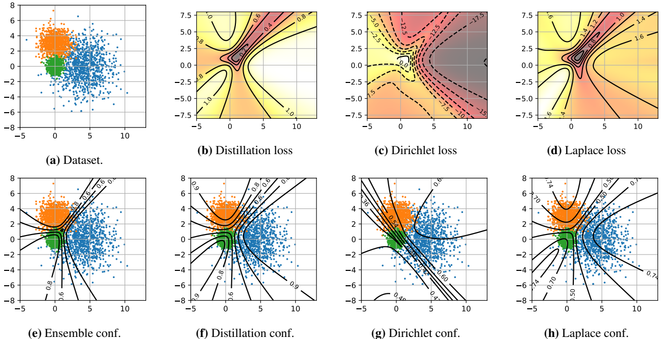
Figure 1: An artificial three-class classification problem with 1000 examples per class. The top row shows the loss surface contours for various distillation approaches; darker colours imply lower losses. The bottom row shows the corresponding confidence contours (the confidence scores are reported on the contour). This shows that Dirichlet-based EDD is unable to learn properly whilst our proposed Laplace L-EDD can imitate an ensemble.
