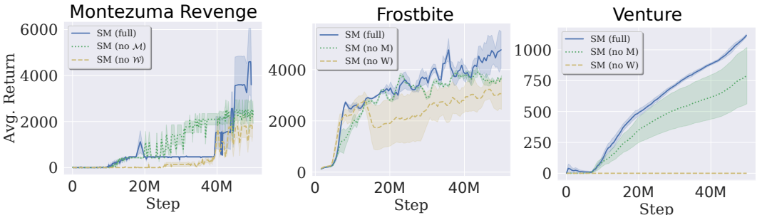
Figure 10: Ablation study: average returns (mean±std.) over 5 runs.
