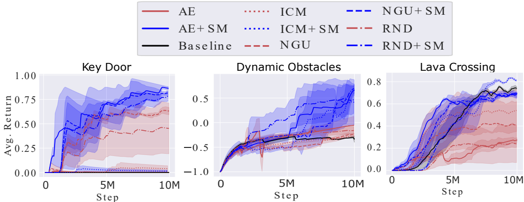
Figure 7: Minigrid’s learning curves over 10 million training steps (mean \pm std. over 5 runs).
