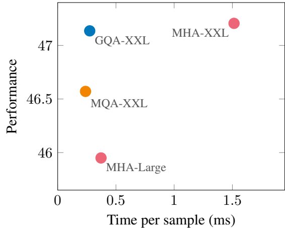
Figure 3: Uptrained MQA yields a favorable trade-off compared to MHA with higher quality and faster speed than MHA-Large, and GQA achieves even better performance with similar speed gains and comparable quality to MHA-XXL. Average performance on all tasks as a function of average inference time per sample for T5-Large and T5-XXL with multi-head attention, and 5% uptrained T5-XXL with MQA and GQA-8 attention.
