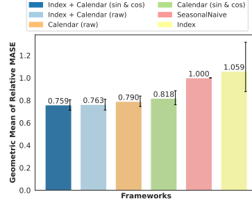
Figure 3: TabPFN-TS performance with different feature combinations. Seasonal Naive is included for reference.
