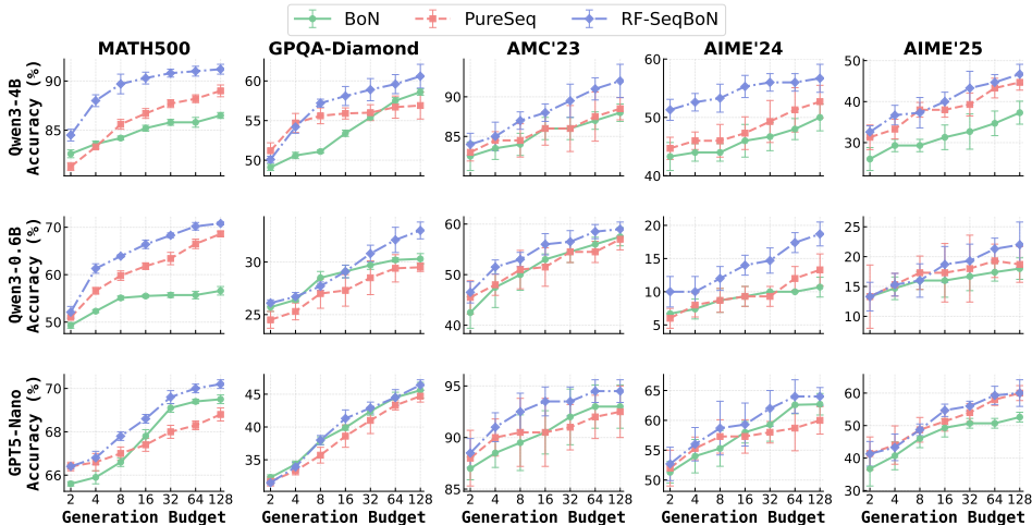
Figure 1: Main results with Qwen3-4B-Instruct ( top ), Qwen3-0.6B-Thinking ( medium ) and GPT5-Nano ( bottom ) foundation models of values with generation budget N . Each column corresponds to one benchmark dataset. The points and error bars show the mean and standard deviation across five repeated experiments, respectively.
