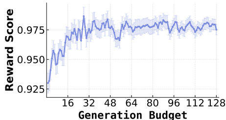
Figure 5: Reward score trend of RF-SeqBoN for the given problem. Points and error bars denote the mean and standard deviation across five repeated experiments.
