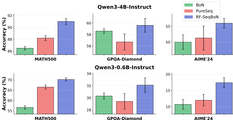
Figure 4: Accuracy comparison for BoN, PureSeq and RF-SeqBoN under the same test-time budget. The bar heights and error bars show the mean and standard deviation from five repeated experiments, respectively. The RF-SeqBoN still dominates the other two in all settings.
