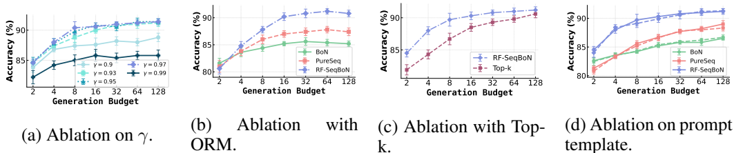
Figure 3: Ablation study results on MATH500 using Qwen3-4B-Instruct as the foundation model. Points denote the mean performance, with error bars representing the standard deviation over five repeated experiments.
