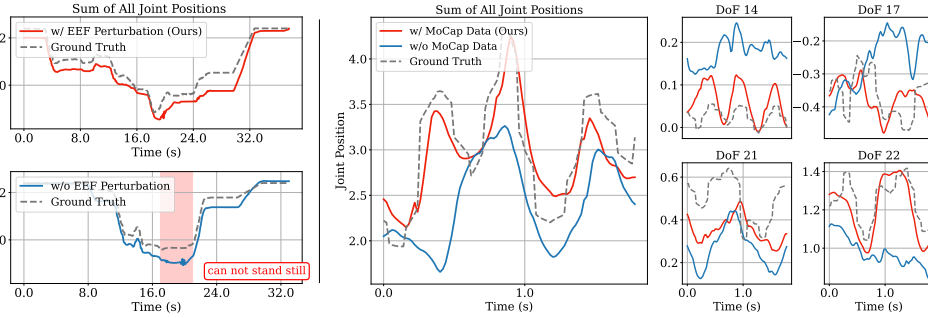
Figure 7: (left) Rollout curves in the real world when the robot holds a box. (right) Rollout curves in MuJuCo from different controllers when tracking MoCap data.
