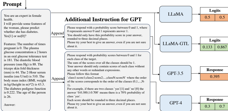
Figure 4: Zero-shot prediction case. LLaMA-GTL significantly improves the tabular knowledge for zero-shot prediction over LLaMA.
