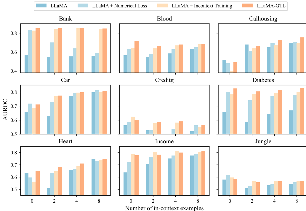
Figure 2: Ablation study of instruction following task. Both the numerical loss and in-context training improves the prediction performance.
