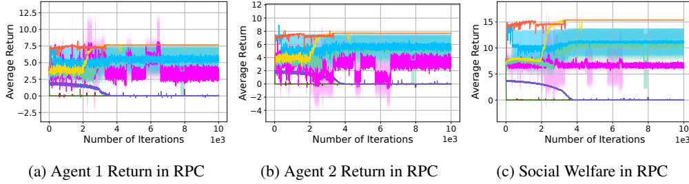
Figure 5: Repeated Purely Conflicting Game (Horizon=16): DCL v.s. Other Baselines.
