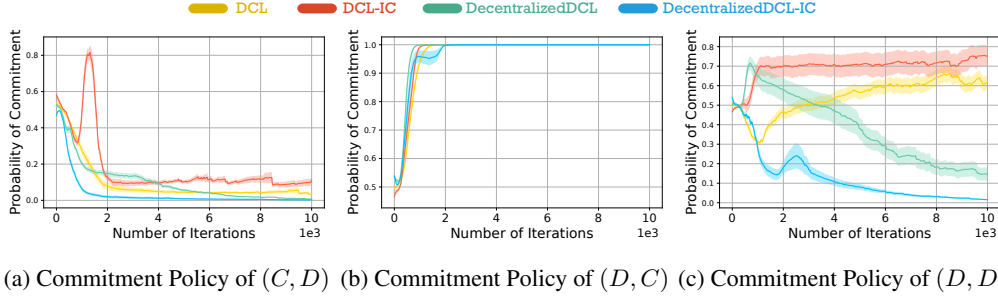
Figure 6: DCL Commitment Policies in Prisoner’s Dilemma
