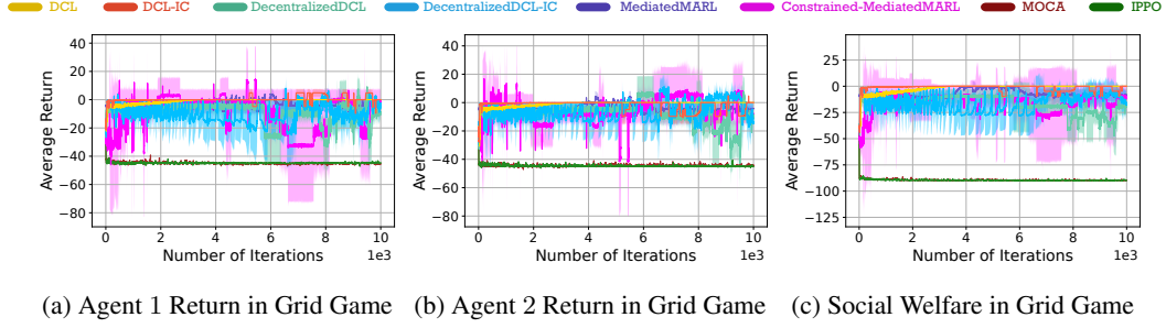
Figure 4: Grid Game (Horizon=16): DCL v.s. Other Baselines.
