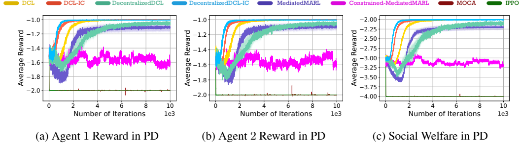
Figure 2: Prisoner's Dilemma: DCL v.s. Other Baselines
