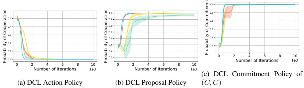
Figure 3: DCL Policies in Prisoner's Dilemma
