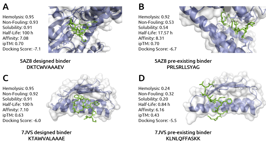
Figure S1: Complex structures of target proteins with pre-existing binders. (A)-(B) 5AZ8 (C)-(D) 7JVS. Each panel shows the complex structure of the target with either an AReURDi-designed binder or its pre-existing binder. For each binder, five property scores are provided, as well as the ipTM score from AlphaFold3 and the docking score from AutoDock VINA. Interacting residues on the target are visualized.
