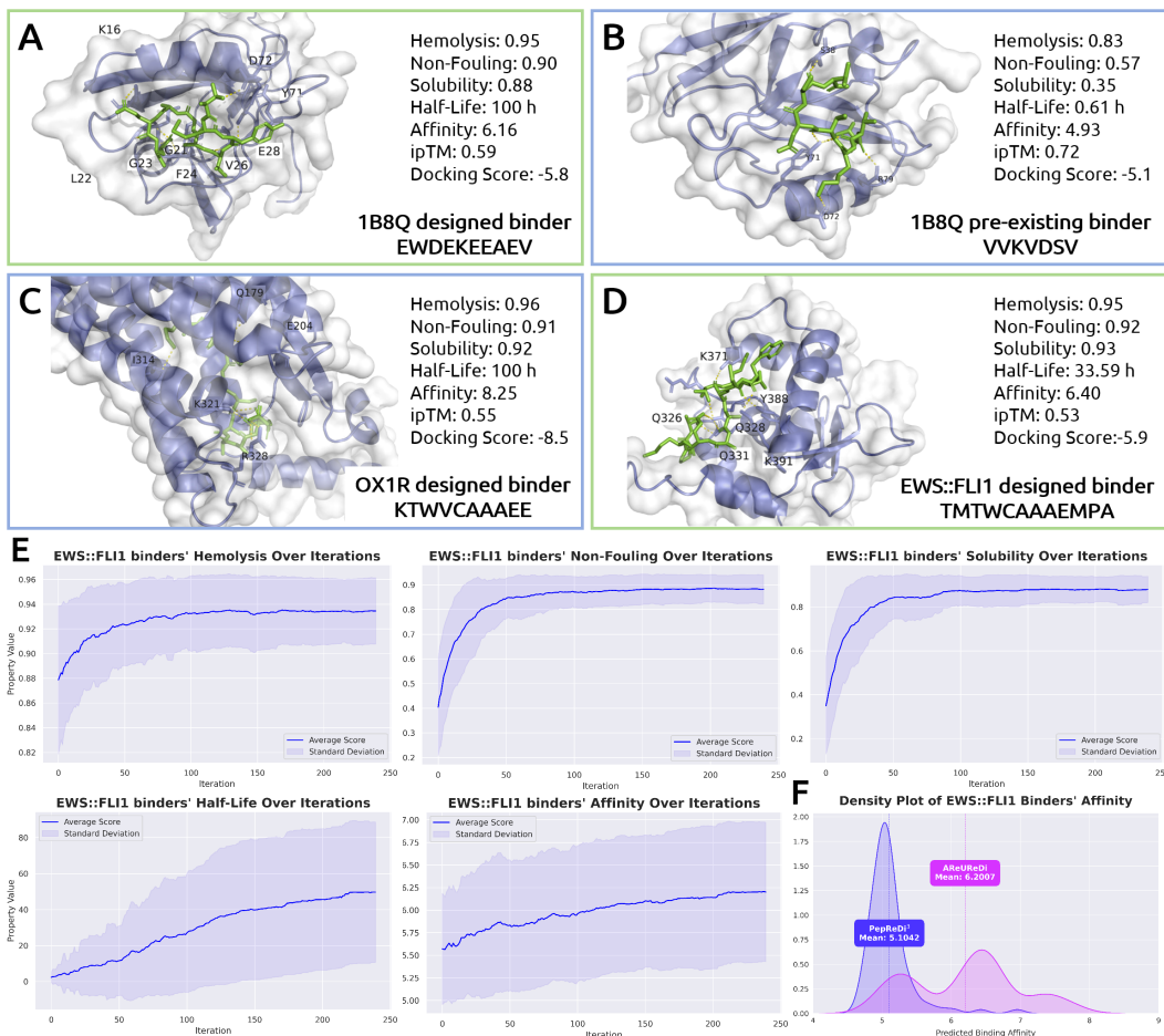
Figure 1: (A), (B) Complex structures of PDB 1B8Q with an AReUReDi-designed binder and its pre-existing binder. (C), (D) Complex structures of OX1R and EWS::FL1I with an AReUReDi-designed binder. Five property scores are shown for each binder, along with the ipTM score from AlphaFold3 and docking score from AutoDock VINA. Interacting residues on the target are visualized. (E) Plots showing the mean scores for each property across the number of iterations during AReUReDi's design of binders of length 12-aa for EWS::FL1I. (F) A density plot illustrating the distribution of predicted property scores for AReUReDi-designed EWS::FL1I binders of length 12-aa, compared to the peptides generated unconditionally by PepReDi 3 .
