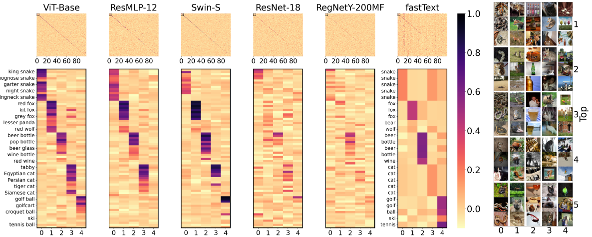
(a) Normalized ICA-transformed embeddings of images and words for five image models and English fastText.
