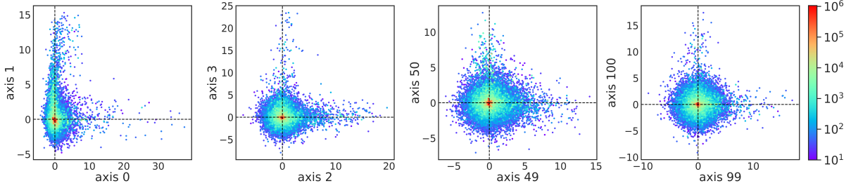
(a) ICA-transformed word embeddings. The axis numbers are sorted by skewness.
