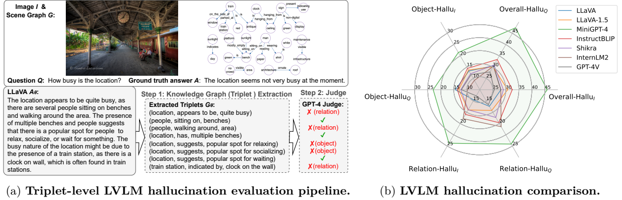
Figure 1: Overview of the unified hallucination evaluation pipeline of Tri-HE. (a) With the provision of images, scene graphs, and questions, knowledge graphs ( i.e. , triplets) are extracted from LVLM responses, which are then judged by an LLM (GPT-4 here). (b) The radar plot showcases the evaluation results among different LVLMs (lower values demonstrate fewer hallucinations).
