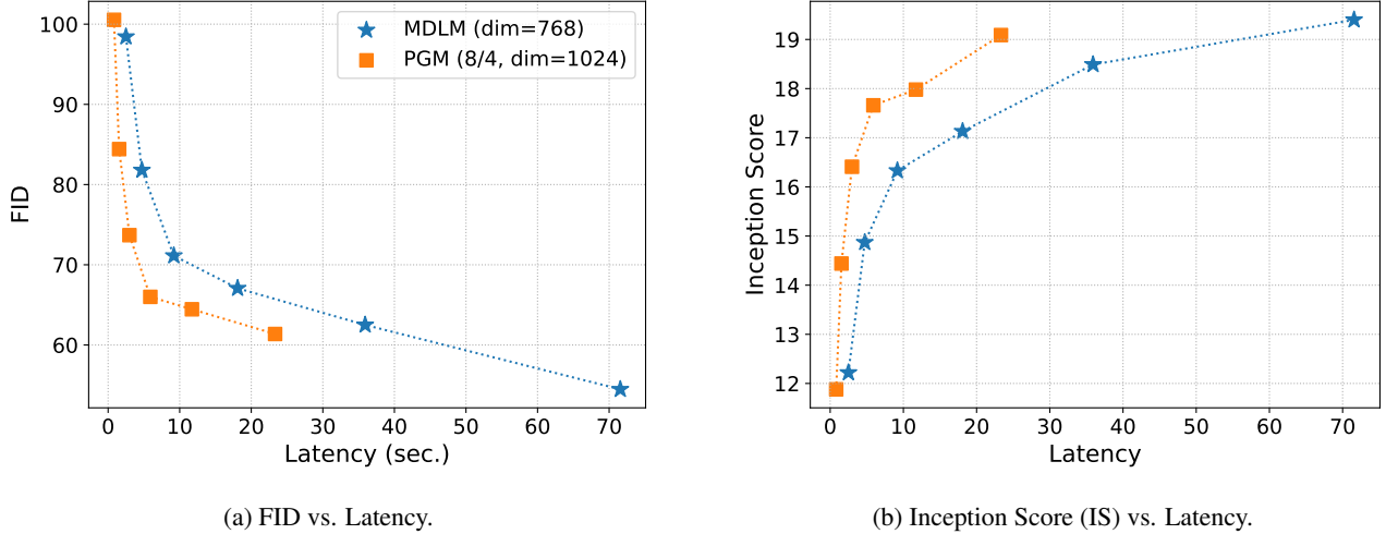
Figure 4. Comparison of the performance of PGMs and MDLMs when modeling discrete image tokens. For a given compute budget, PGMs outperform MDLMs. Note that we do not target state-of-the-art result in this experiment, rather we compare the regular MDLM and PGM that were used in experiments on text.
