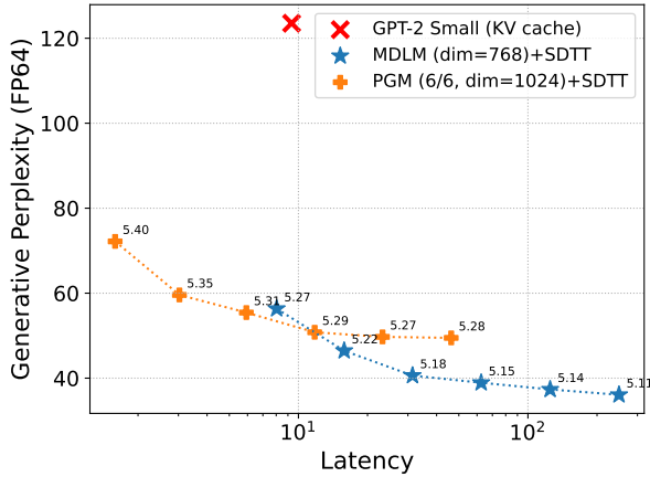
(a) Generative PPL vs. Latency.
