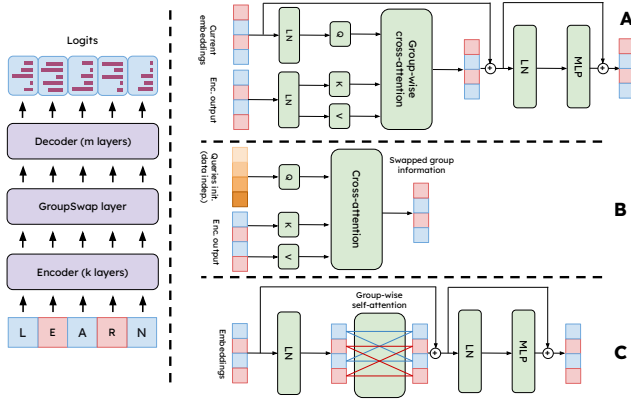
Figure 3. PGM-compatible transformer architecture. RoPE (Su et al., 2023) is applied before every attention layer but not shown for clarity. (A) Decoder layer with cross-attention to the encoder output and no self-attention between tokens. (B) GroupSwap layer that exchanges information between group 0 and group 1 positions, enabling each group to make predictions based on tokens from the other group. (C) Encoder layer with sparse, group-wise self-attention.
