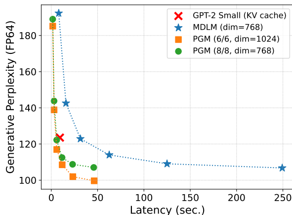
Figure 1. Latency results: PGM (ours) achieves better generative perplexity and at least 5x improvements in latency compared to MDLM on OpenWebText (Gokaslan & Cohen, 2019). All sampling uses power-of-2 step counts. Standard models are evaluated with 32 to 1024 steps, while the model distilled with SDTT uses from 8 to 1024 steps. The improvements come from our specialized neural network architecture.
