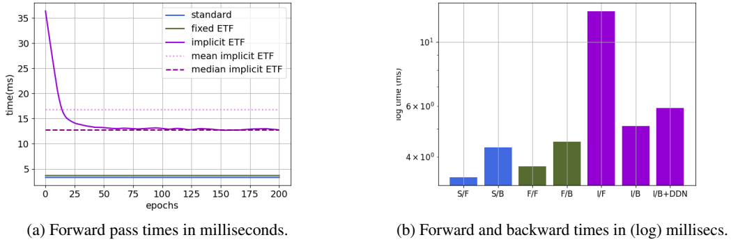
Figure 16: CIFAR10 computational cost results on ResNet-18. In (a), we plot the forward pass time for each method. For the implicit ETF method, which has dynamic computation times, we also include the mean and median time values. In (b), we plot the computational cost for each forward and backward pass across methods. For the implicit ETF forward pass, we have taken its median time. The notation is as follows: S/F = Standard Forward Pass, S/B = Standard Backward Pass, F/F = Fixed ETF Forward Pass, F/B = Fixed ETF Backward Pass, I/F = Implicit ETF Forward Pass, and I/B = Implicit ETF Backward Pass.
