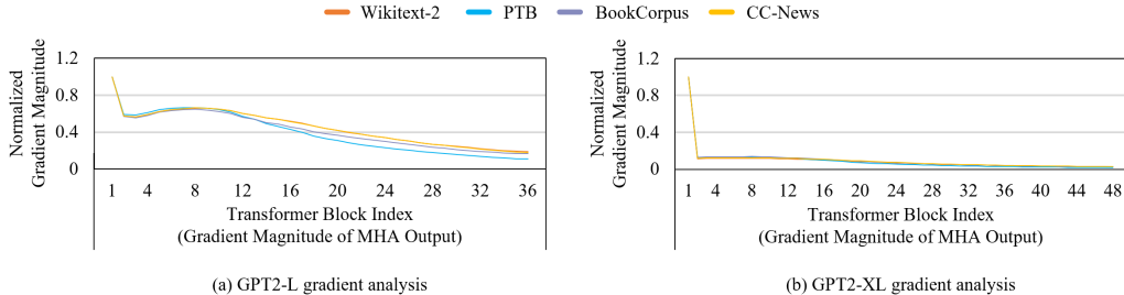
Figure 13: Normalized gradient magnitude of the MHA outputs across Transformer blocks in GPT-2 774M and 1.5B for different datasets. the x-axis represents the block index.
