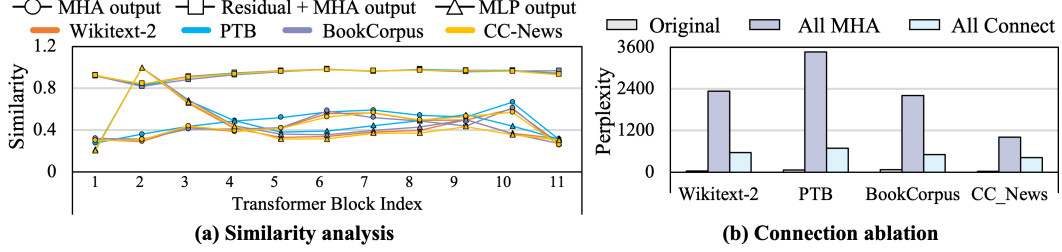
Figure 3: Motivation for reconfiguring MHA-MLP connections. (a) CKA similarity analysis across successive GPT-2 blocks. The x-axis indicates the block index, and the y-axis shows the similarity between consecutive MHA outputs, Residual+MHA outputs (i.e., MLP inputs), and MLP outputs. (b) Connection ablation results measured by perplexity. Original denotes the unaltered model, All MHA removes all MHA layer, and All Connect removes all direct MHA-MLP connections.
