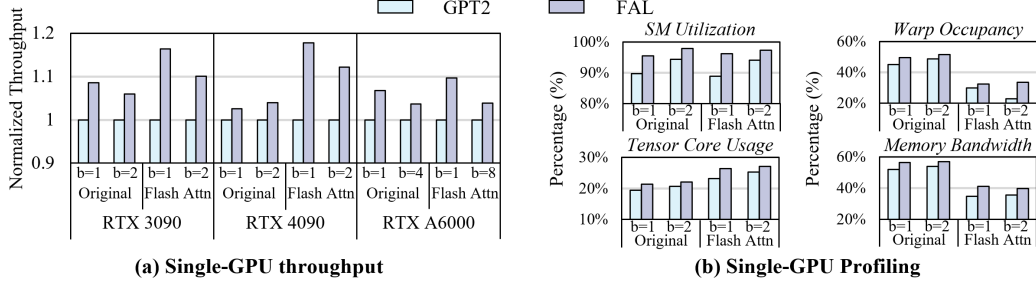
Figure 8: Single-GPU throughput comparison between GPT2 and FAL. (a) Normalized throughput (tokens/sec). (b) Analysis of throughput gains on RTX 3090.
