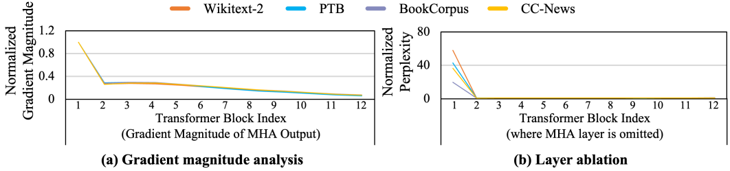
Figure 4: The crucial role of the first attentions. (a) Normalized gradient magnitude of the MHA outputs across Transformer blocks in GPT-2 for different datasets. The x-axis represents the block index. (b) Layer ablation results measured by perplexity. The x-axis indicates the index of the transformer block from which the MHA is omitted.
