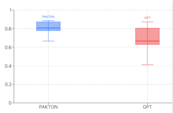
Figure 5: Comparative analysis of PAKTON vs. GPT-4o based on the G-EVAL framework across different criteria. Distribution of the aggregated scores across all criteria.
