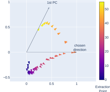
Figure 6: Projections of the feature directions extracted at each layer (i.e. \hat{d}_{\text{feat}}^i ) on the steering plane for QWEN2.5-7B-INSTRUCT.
