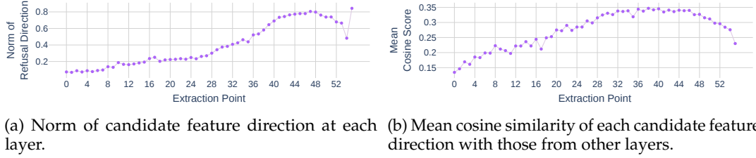
Figure 5: Statistics of refusal direction candidate for QWEN2.5-7B-INSTRUCT.
