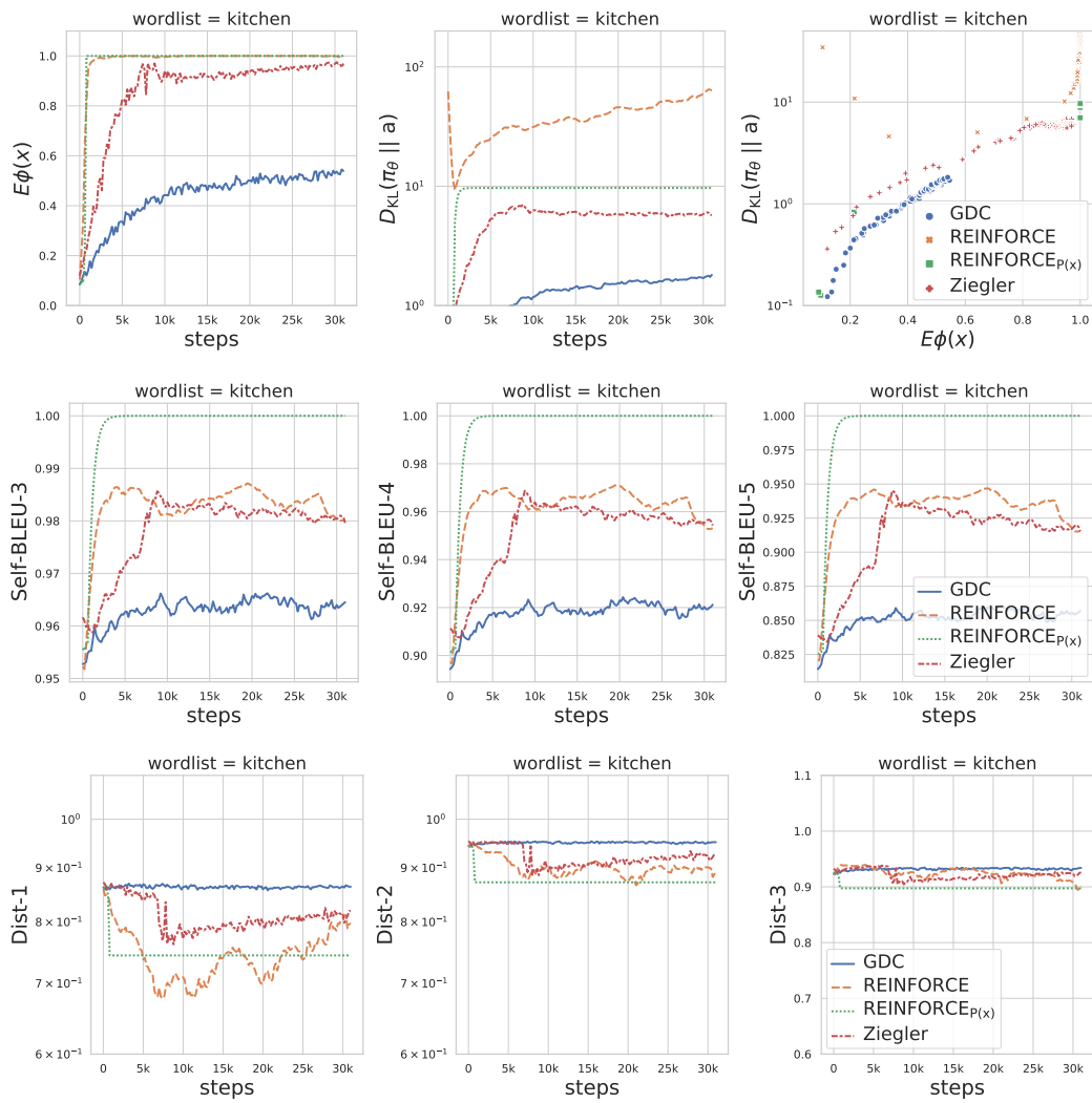
Figure 27: Line plot of different evaluation metrics against the training steps when controlling for the kitchen word-list.
