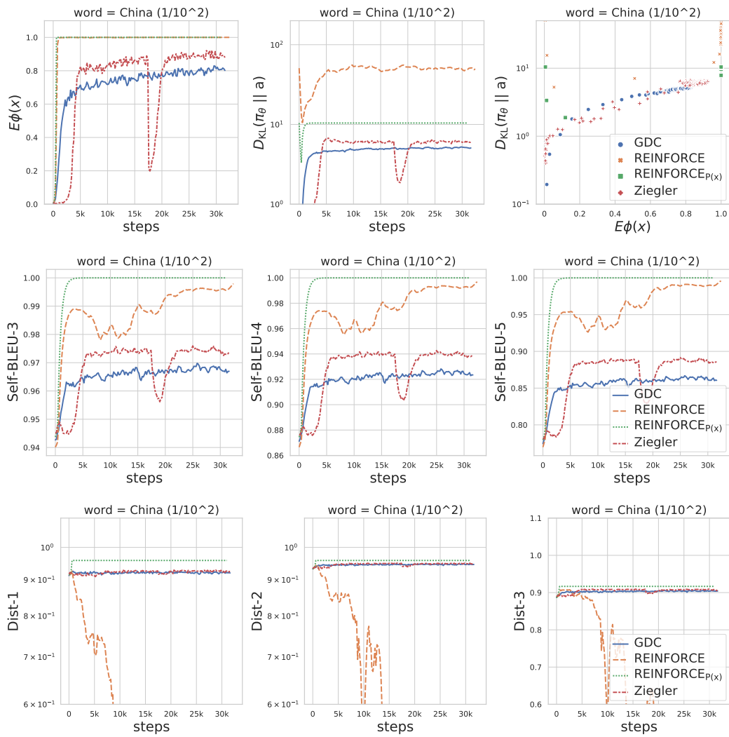
Figure 25: Line plot of different evaluation metrics against the training steps when controlling for the word “China” (with initial occurrence probability of 1/100) as a single-word constraint.
