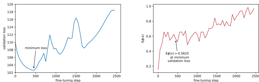
Figure 7: Supervised experiment when fine-tuning GPT-2 on a corpus of sentences containing the word “amazing”. Left: validation loss development during fine-tuning. Right: percentage of samples generated using the fine-tuned model and containing the word “amazing”. Here, the best model according to the validation loss is only able to achieve \mathbb{E}\phi(x) = 0.5625 . Higher values of \mathbb{E}\phi(x) tend to occur with higher validation loss, i.e. when overfitting.
