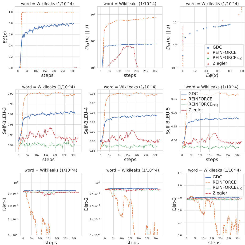
Figure 18: Line plot of different evaluation metrics against the training steps when controlling for the word “wikileaks” (with initial occurrence probability of 1/10000 ) as a single-word constraint.
