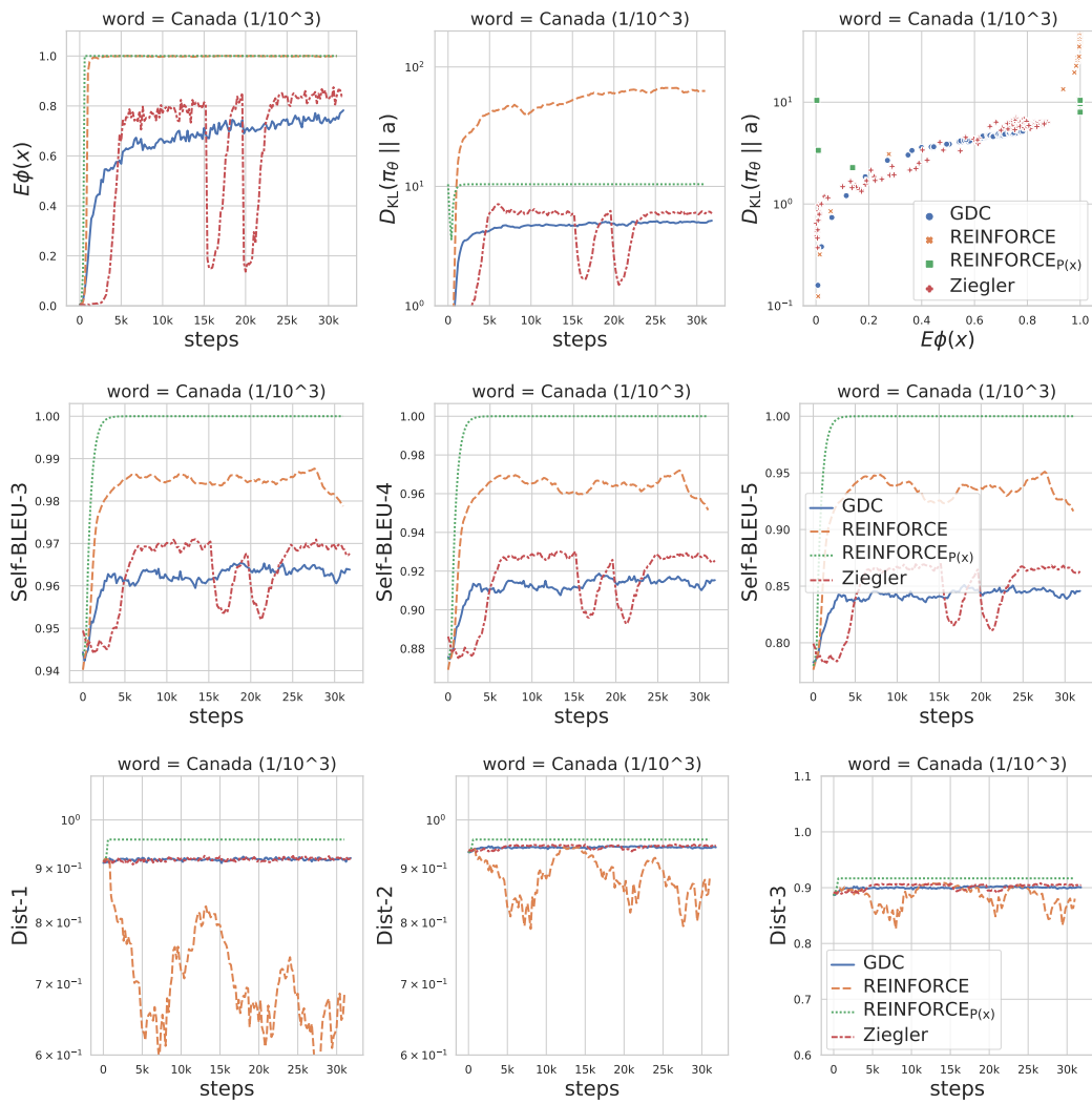
Figure 24: Line plot of different evaluation metrics against the training steps when controlling for the word “Canada” (with initial occurrence probability of 1/1000) as a single-word constraint.
