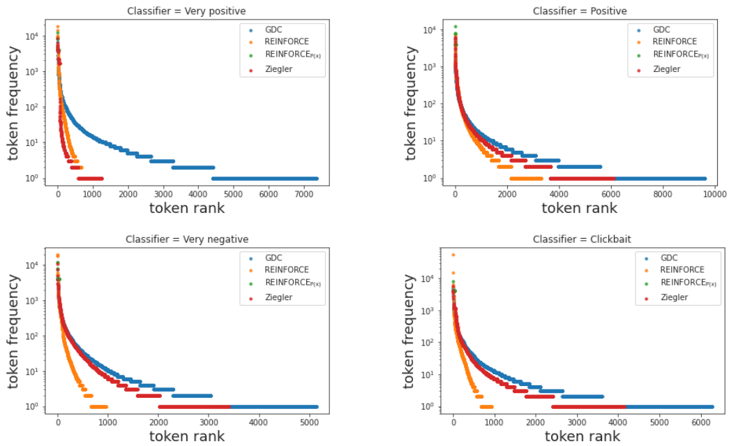
Figure 37: Token frequency against token rank for classifier-based constraints. Longer tail means more diverse generations.
