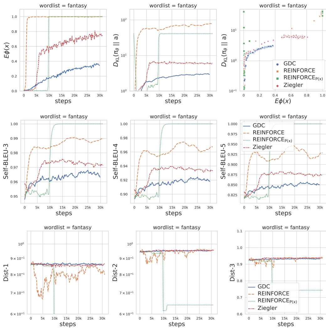
Figure 28: Line plot of different evaluation metrics against the training steps when controlling for the fantasy word-list.
