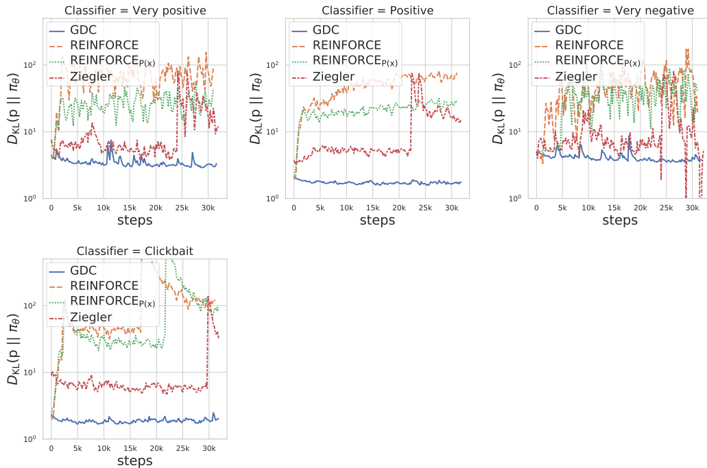
Figure 17: D_{\text{KL}}(p, \pi_{\theta}) against the training steps for GDC and the three baselines introduced in section 3.2 for classifier-based control. Curves are displayed using 4 different classifiers: very positive, positive, and very negative sentiment, and click-bait. GDC exhibits much better convergence behaviour than the other baselines, showing its superiority in approximating the desired distribution p .
