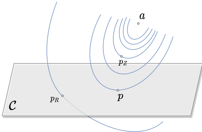
Figure 8: Case of a pointwise binary requirement r(x) = 1 : comparison with Reinforce and Ziegler. The curves correspond to different D_{\text{KL}}(\cdot, a) levels. The manifold \mathcal{C} is the set of distributions c s.t. c(x) > 0 \rightarrow r(x) = 1 , or, equivalently s.t. \mathbb{E}_{x \sim c} r(x) = 1 . The curved lines represent increasing levels of the KL divergence D_{\text{KL}}(q, a) . According to Reinforce, any distribution p_R s.t. \mathbb{E}_{x \sim p_R} r(x) = 1 , that is, any distribution on \mathcal{C} , is optimal. According to Ziegler, to each temperature \beta > 0 is associated an optimal distribution p_Z = \arg \min_q \beta D_{\text{KL}}(q, a) - \mathbb{E}_{x \sim q} r(x) , which does not directly lie on \mathcal{C} — this is because, as indicated in (Ziegler et al., 2019), this distribution is of the form p_Z(x) \propto a(x)e^{r(x)/\beta} , giving positive probability to all x ’s in the support of a , including to points not lying on \mathcal{C} . Our own optimal p does lie on \mathcal{C} by definition, while minimizing the KL divergence from a .
