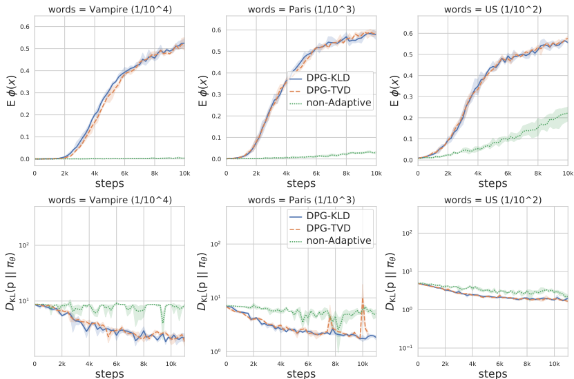
Figure 6: Ablation experiment elaborating the effectiveness of the adaptive step in the DPG algorithm explained in section 2. We compare three adaptivity variants, based on the KL divergence (DPG-KLD), on the TVD distance (DPG-TVD) and with no adaptation. We find similar convergence rates for both KLD and TVD adaptive DPG compared to a much slower convergence without adaptation.
