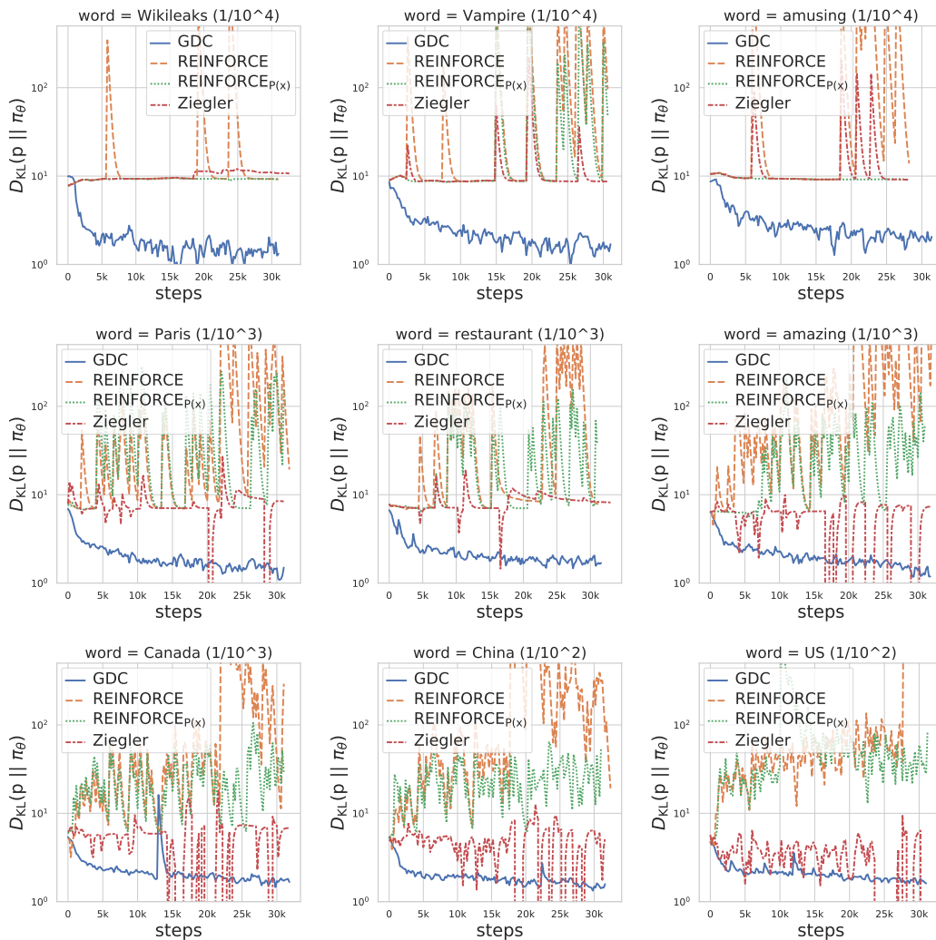
Figure 15: D_{KL}(p, \pi_\theta) against the training steps for GDC and the three baselines introduced in section §3.2 for the single-word control task. Curves are displayed for nine different single-word constraints of varying rarity levels (1/100, 1/1000, 1/10000). GDC exhibits much better convergence behaviour than the other baselines, showing its superiority in approximating the desired distribution p .
