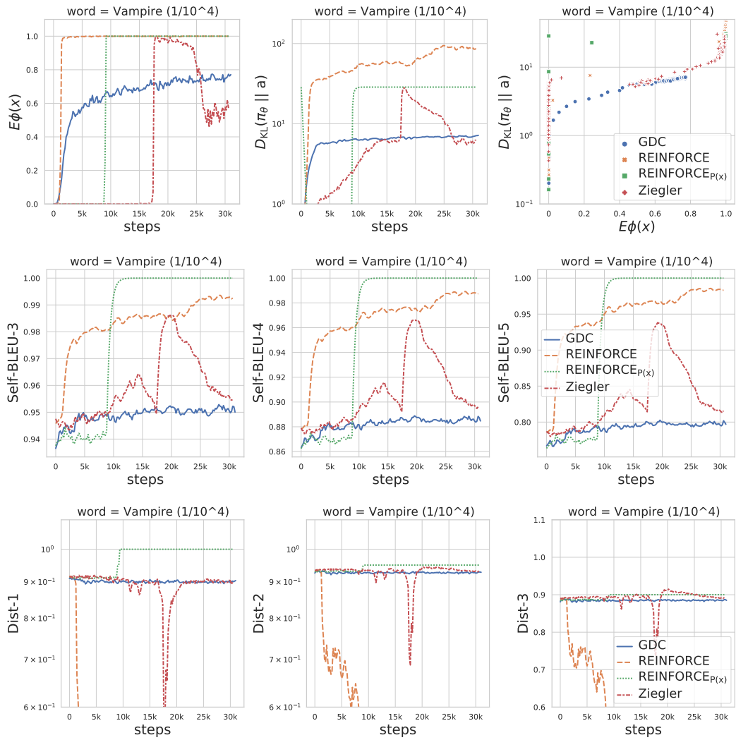
Figure 19: Line plot of different evaluation metrics against the training steps when controlling for the word “vampire” (with initial occurrence probability of 1/10000 ) as a single-word constraint.
