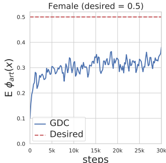
Figure 9: Exp1: Single Distributional Constraint. Balancing demographics can be represented easily through distributional constraints. By using a constraint such as \mathbb{E}_{x \sim p} \phi_{female}(x) = 0.5 , we can target balancing the female biographies in the distribution of all generations. Note that a point-wise objective \mathbb{E}_{x \sim p} \phi_{female}(x) = 1.0 would maximize the presence of female biographies at the expense of other demographics, inducing bias in the opposite direction. The plot shows how \mathbb{E}_{x \sim p} \phi_{female}(x) evolves towards the defined expectation: GDC is able to reduce the bias of GPT-2 bio to obtain 36.7% female biographies rather than just 7%.
