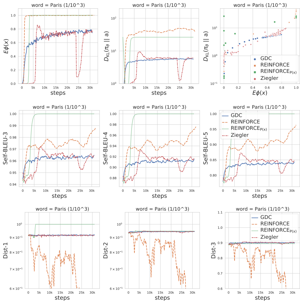
Figure 21: Line plot of different evaluation metrics against the training steps when controlling for the word “Paris” (with initial occurrence probability of 1/1000) as a single-word constraint.
