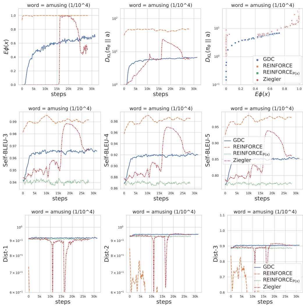
Figure 20: Line plot of different evaluation metrics against the training steps when controlling for the word “amusing” (with initial occurrence probability of 1/10000) as a single-word constraint.
