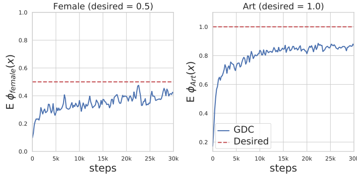
Figure 11: Exp3: Hybrid constraints In this experiment, we specify two types of constraints: pointwise with \mathbb{E}\phi_{art}(x) = 1.0 and distributional with \mathbb{E}\phi_{female}(x) = 0.5 (henceforth Hybrid). GDC in a single training procedure is able to increase the expectation of biographies about females from 7.4% to 36.6% and Art professions from 11.4% to 88.6%.
