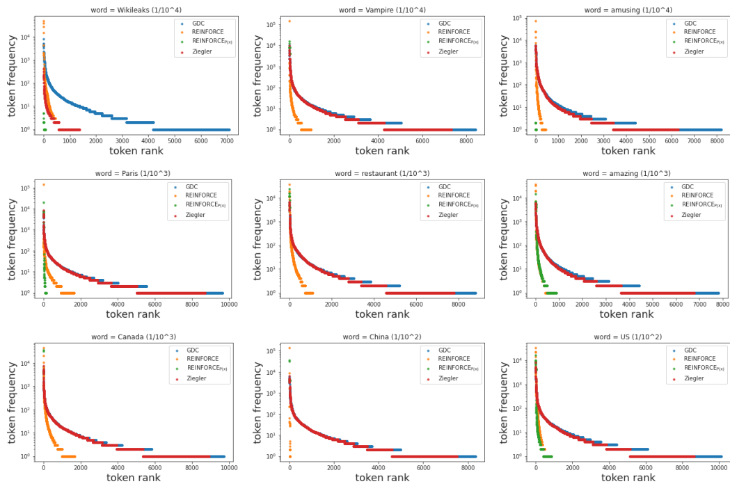
Figure 35: Token frequency against token rank for single-word constraints. Longer tail means more diverse generations.
