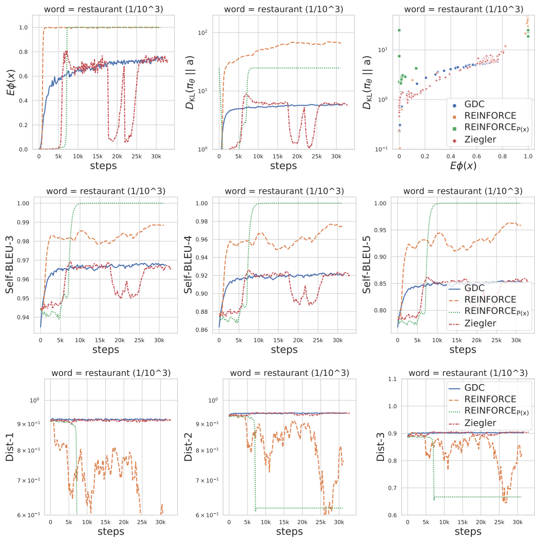
Figure 22: Line plot of different evaluation metrics against the training steps when controlling for the word “restaurant” (with initial occurrence probability of 1/1000) as a single-word constraint.
