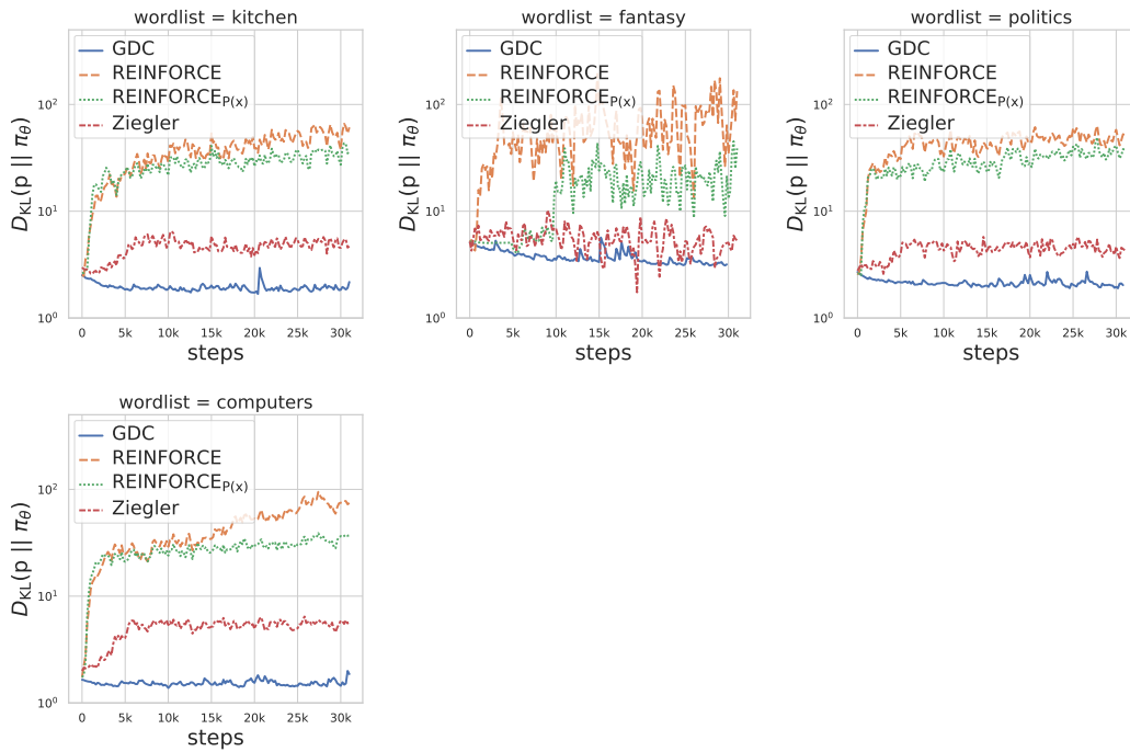
Figure 16: D_{\text{KL}}(p, \pi_{\theta}) against the training steps for GDC and the three baselines introduced in section 3.2 for word-list constraints. Curves are displayed for 4 word-lists: kitchen , fantasy, politics, computers. GDC exhibits much better convergence behaviour than the other baselines, showing its superiority in approximating the desired distribution p .
