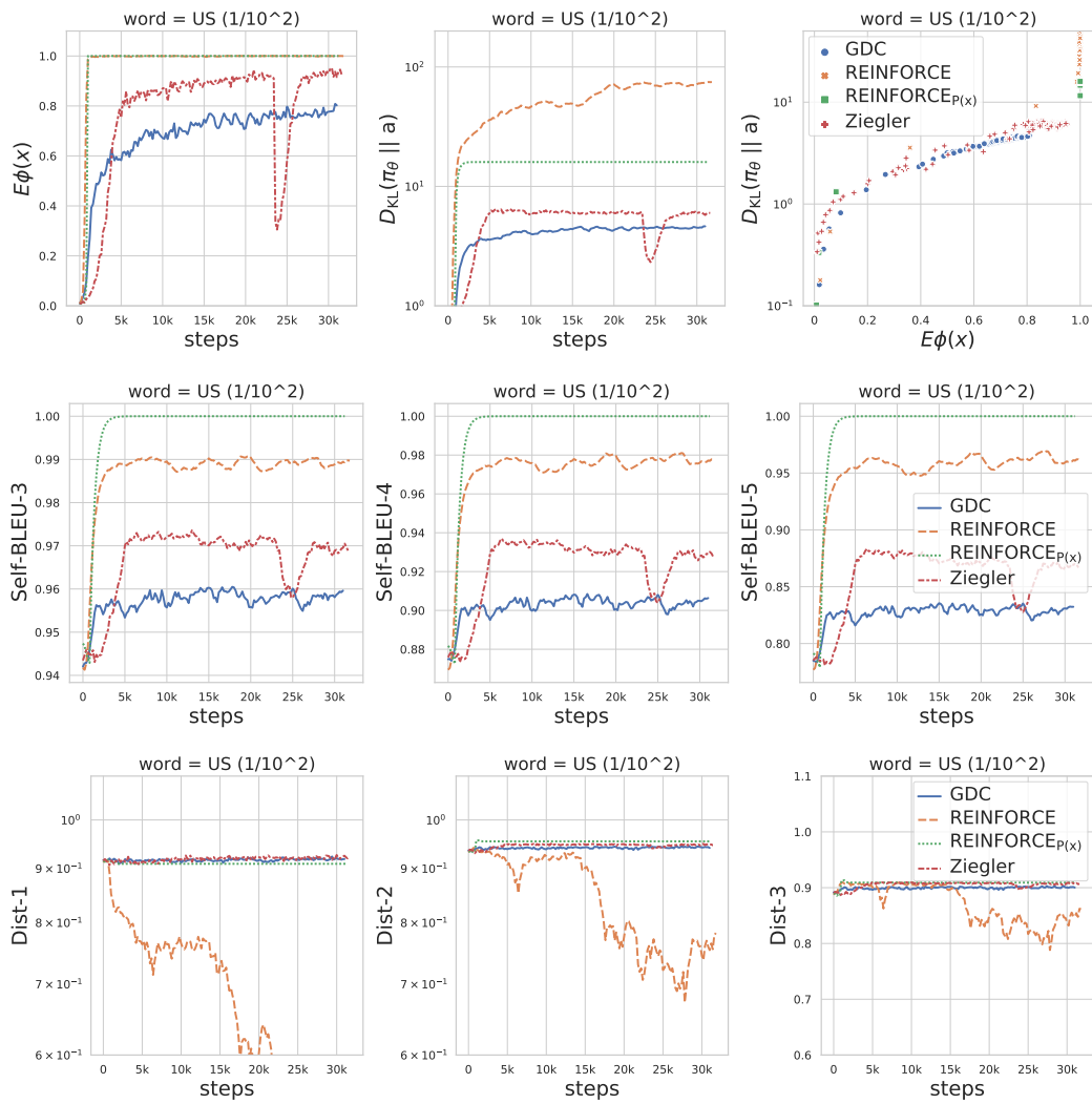
Figure 26: Line plot of different evaluation metrics against the training steps when controlling for the word “US” (with initial occurrence probability of 1/100) as a single-word constraint.
