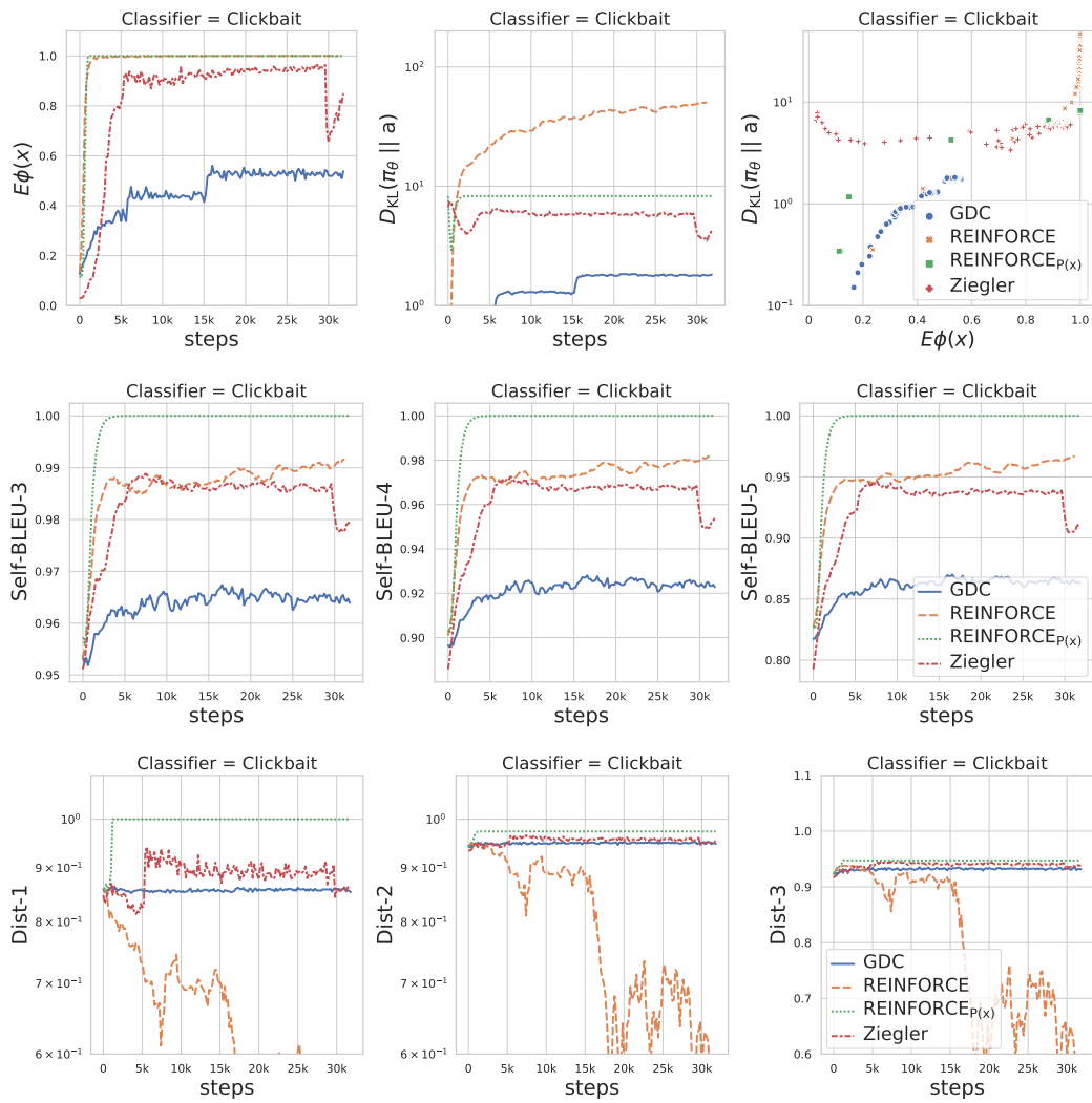
Figure 34: Line plot of different evaluation metrics against the training steps for click-bait classifier-based control with.
