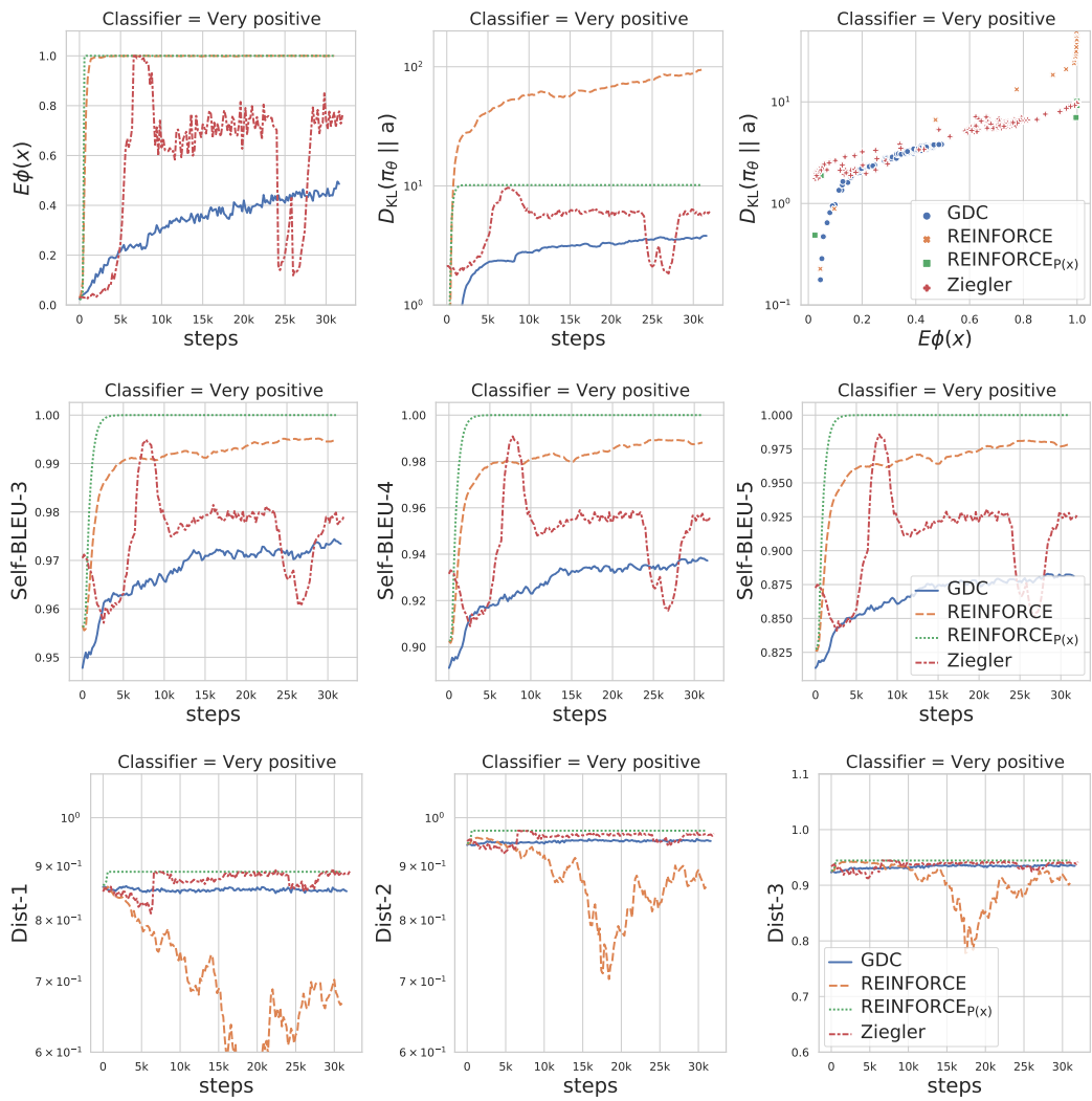
Figure 31: Line plot of different evaluation metrics against the training steps when controlling for the politics word-list.
