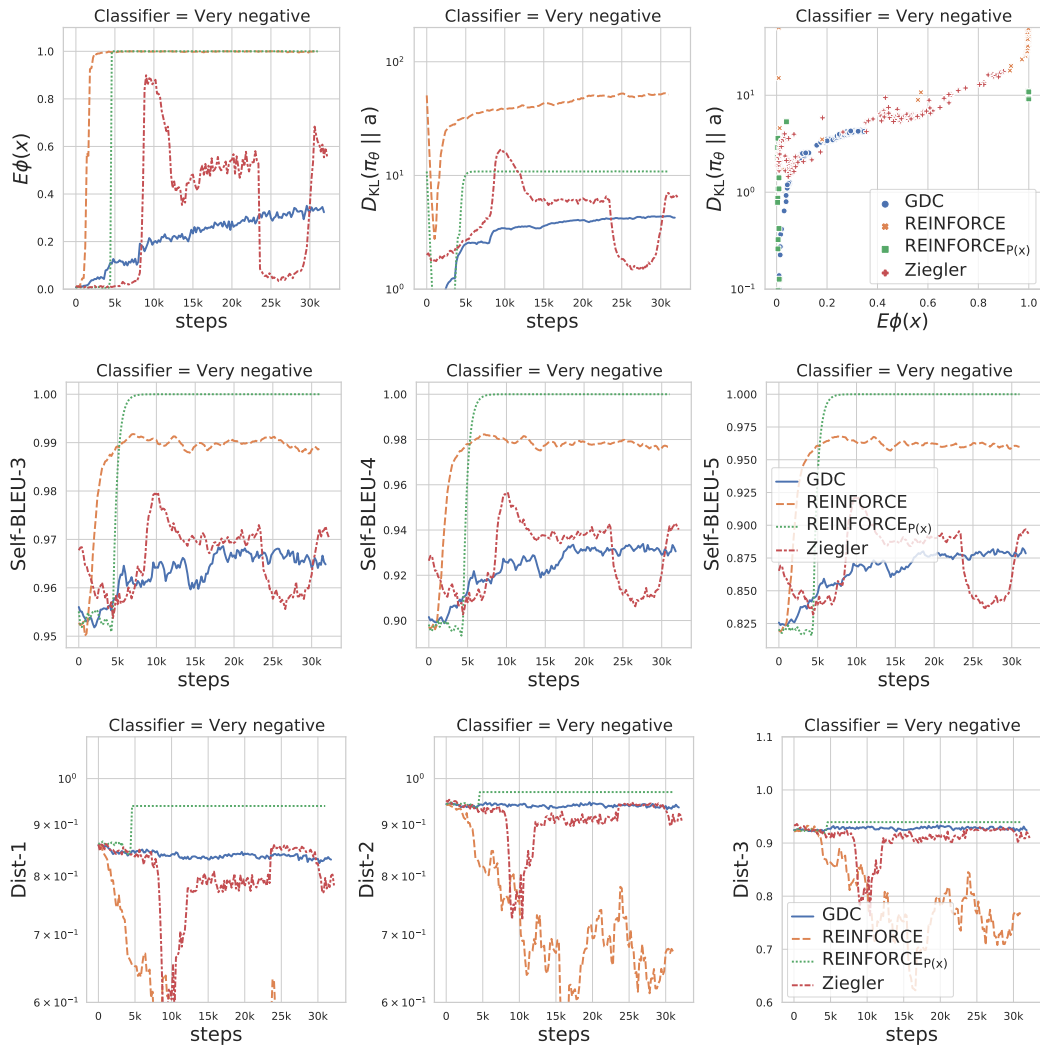
Figure 33: Line plot of different evaluation metrics against the training steps for very negative sentiment classifier-based control with.
