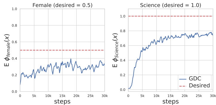
Figure 14: Exp6: Hybrid constraints. In this experiment, we specify two types of constraints: pointwise with \mathbb{E}\phi_{science}(x) = 1.0 and distributional with \mathbb{E}\phi_{female}(x) = 0.5 . GDC in a single training procedure is able to increase the expectation of biographies about females from 7.4% to 28.8% and Science professions from 1.2% to 74.7%.
