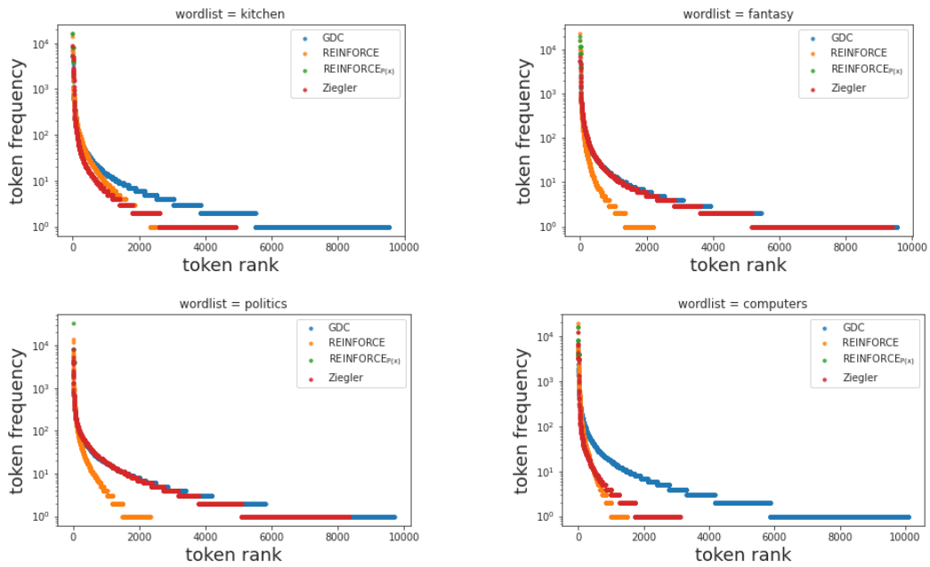
Figure 36: Token frequency against token rank for word-list constraints. Longer tail means more diverse generations.
