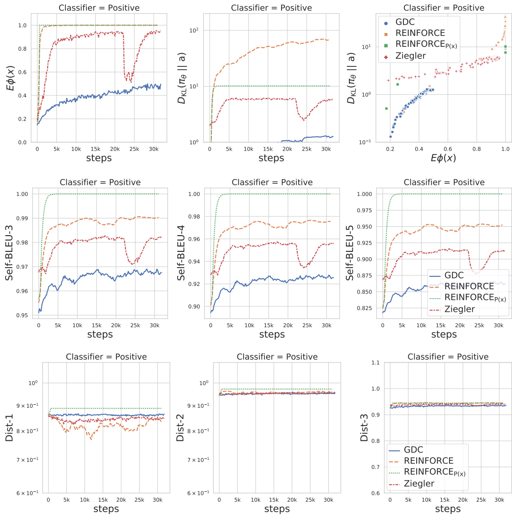
Figure 32: Line plot of different evaluation metrics against the training steps for positive sentiment classifier-based control with.
