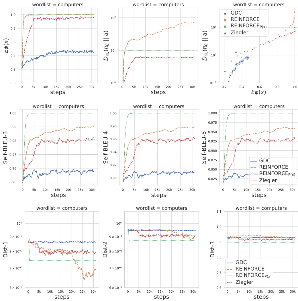
Figure 30: Line plot of different evaluation metrics against the training steps when controlling for the com-puters word-list.
