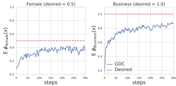
Figure 13: Exp5: Hybrid constraints. In this experiment, we specify two types of constraints: pointwise with \mathbb{E}\phi_{business}(x) = 1.0 and distributional with \mathbb{E}\phi_{female}(x) = 0.5 . GDC in a single training procedure is able to increase the expectation of biographies about females from 7.4% to 37.7% and Business professions from 10.1% to 82.4%.
