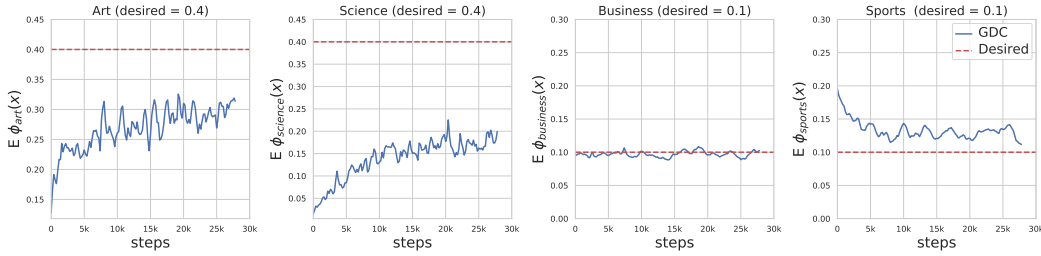
Figure 10: Exp2: Multiple Distributional Constraints This experiment demonstrates the flexibility of GDC in dealing with several distributional constraints at once, even when these constraints have different objectives (increase, decrease, or keep fixed). We challenge the flexibility of GDC by setting four distributional constraints with four arbitrary expectation values targeting \mathbb{E}\phi_{science} and \mathbb{E}\phi_{art} at 40% and \mathbb{E}\phi_{sports} and \mathbb{E}\phi_{business} at 10%. In the figure, from left to right, we can note the increase of \mathbb{E}\phi_{science} and \mathbb{E}\phi_{art} from 1.5% to 20.3% and from 10% to 31.6% respectively. Interestingly, the initial \mathbb{E}\phi_{business} of GPT-2 bio (10.9%) is already very close to the desired expectation (10%), and we can see that during the course of the training, GDC keeps this value fixed as it is already satisfying the corresponding target distributional constraint. \mathbb{E}\phi_{sports} initially starts higher than the target distributional constraint 10%, and we can note that GDC succeeds to reduce it from 19.6% to 11.9%.
