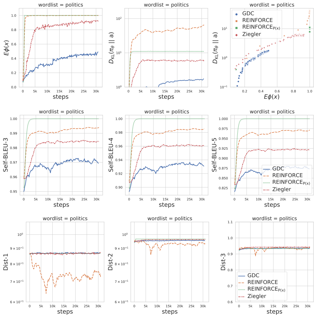
Figure 29: Line plot of different evaluation metrics against the training steps when controlling for the politics word-list.
