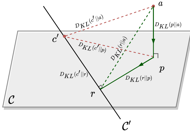
Figure 5: Transitivity of Information Projection (aka Generalized MaxEnt).
