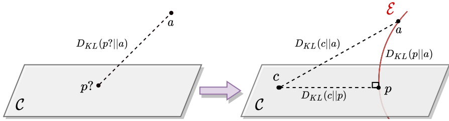
Figure 1: From MaxEnt to EBM through Information Geometry. The Generalized MaxEnt specification (left panel) is looking for a distribution p that lies on the moment constraints manifold \mathcal{C} and that minimizes the forward KL D_{\text{KL}}(p, a) . The solution is provided by Information Geometry: (1) build the exponential family \mathcal{E} determined by a and \phi , (2) p lies at the intersection between \mathcal{C} and \mathcal{E} , (3) for any distribution c satisfying the constraints, the “Pythagorean identity” holds: D_{\text{KL}}(c||a) = D_{\text{KL}}(c||p) + D_{\text{KL}}(p||a) ; in particular p is unique.
