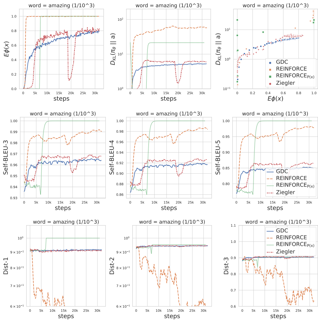
Figure 23: Line plot of different evaluation metrics against the training steps when controlling for the word “amazing” (with initial occurrence probability of 1/1000) as a single-word constraint.
