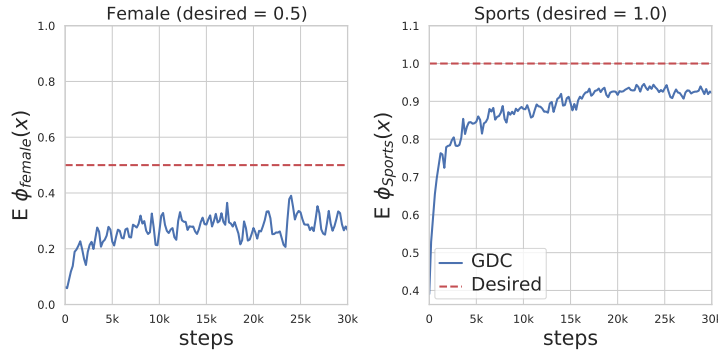
Figure 12: Exp4: Hybrid constraints. In this experiment, we specify two types of constraints: pointwise with \mathbb{E}\phi_{sports}(x) = 1.0 and distributional with \mathbb{E}\phi_{female}(x) = 0.5 . GDC in a single training procedure is able to increase the expectation of biographies about females from 7.4% to 31.9% and Sports professions from 17.5% to 92.9%.
