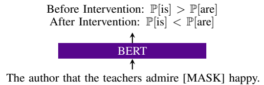
Figure 1: Illustration of our counterfactual intervention (above) and our verb conjugation test (below).
