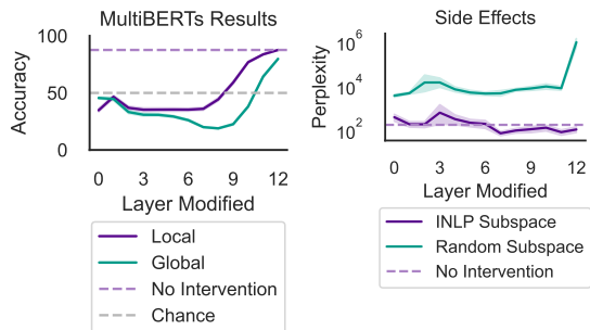
Figure 5: Left: Similar results are obtained when repeating the experiment using the MultiBERT models. Right: Intervention on number-neutral words has no adverse effect on perplexity. Error bands represent 95% confidence intervals obtained from 5 samplings of INLP training vectors.
