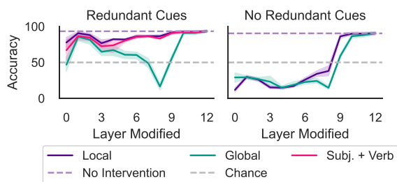
Figure 3: The linear encoding of subject number spreads to positions other than the subject when there are redundant cues to subject number, such as an embedded verb . In the “subj. + verb” condition, intervention is applied to the subject and embedded verb positions. Error bands represent 95% confidence intervals obtained from 5 samplings of INLP training vectors.
