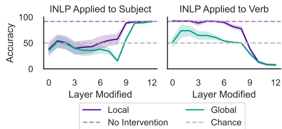
Figure 4: Conjugation accuracy drops to 7.6% when intervening on layer 12 with INLP training vectors extracted from the verb position (right) instead of the subject position (left). Error bands represent 95% confidence intervals obtained from 5 samplings of INLP training vectors.
