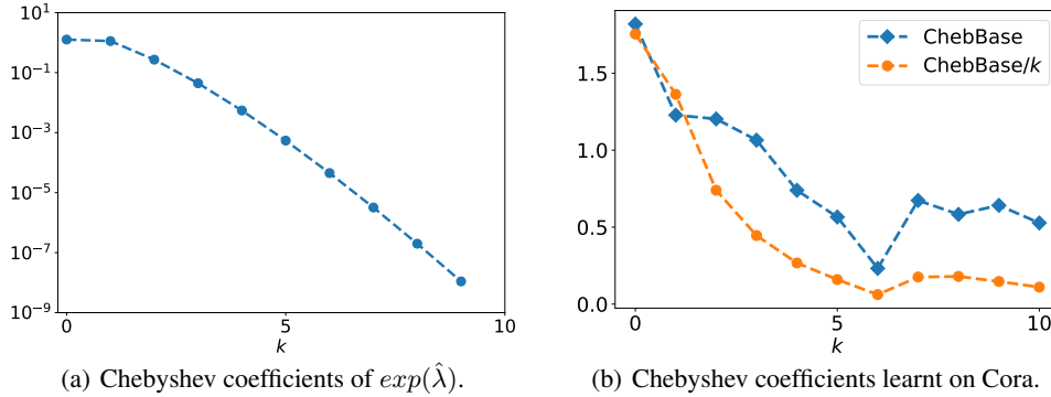
Figure 1: Illustrations of the Chebyshev expansion’s coefficients of \exp(\hat{\lambda}) and the Chebyshev coefficients learnt by ChebBase and ChebBase/ k on Cora.
